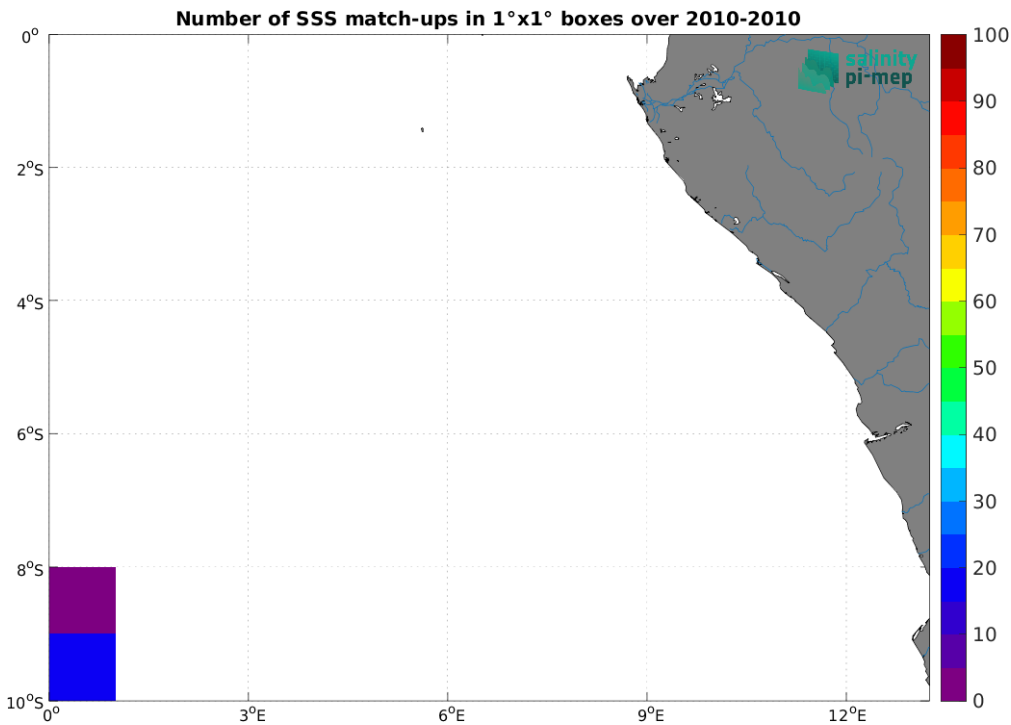
Figure 5: Number of SSS match-ups between TSG (SAMOS) SSS and the SMOS SSS L4 v1 - Monthly (CMEMS-CNR) SSS product for the Congo river plume Pi-MEP region over 1°x1° boxes and for the full satellite product period.
