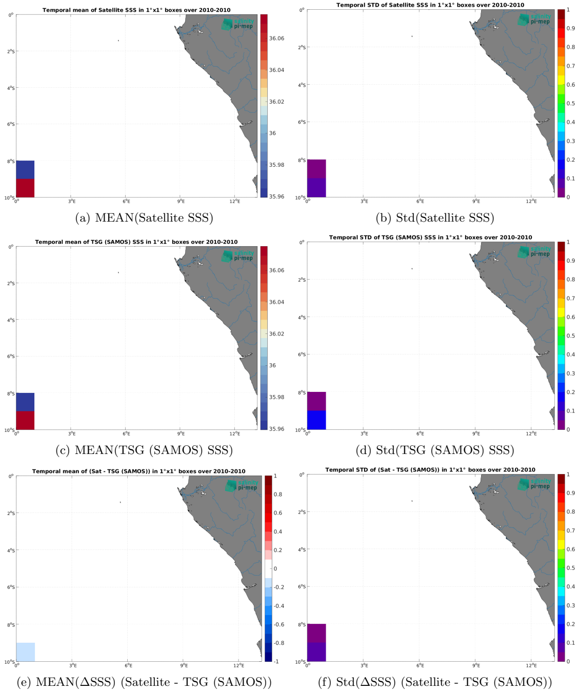
Figure 7: Temporal mean (left) and Std (right) of SSS from SMOS SSS L4 v1 - Monthly (CMEMS-CNR) (top), TSG (SAMOS) (middle), and of \Delta SSS (Satellite - TSG (SAMOS)). Only match-up pairs are used to generate these maps.
