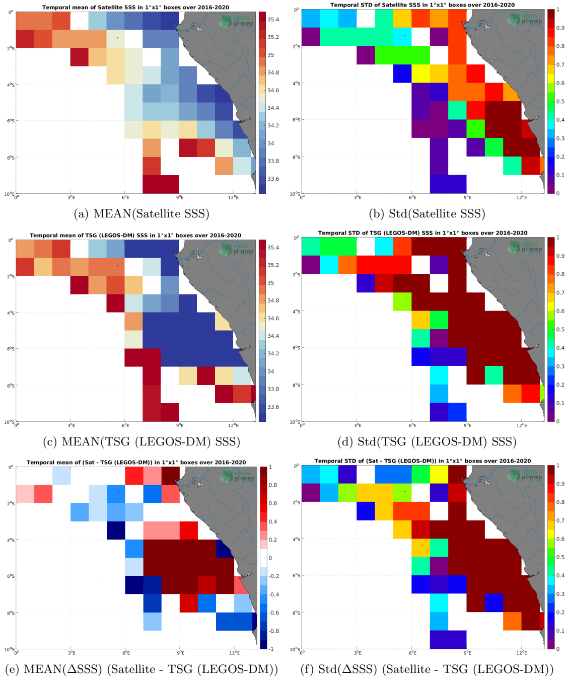
Figure 6: Temporal mean (left) and Std (right) of SSS from SMOS SSS L4 v1 - Monthly (CMEMS-CNR) (top), TSG (LEGOS-DM) (middle), and of \Delta SSS (Satellite - TSG (LEGOS-DM)). Only match-up pairs are used to generate these maps.
