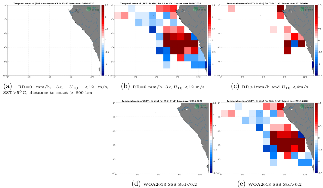
Figure 12: Temporal mean gridded over spatial boxes of size 1^\circ \times 1^\circ of \Delta SSS (SMOS SSS L4 v1 - Monthly (CMEMS-CNR) - TSG (LEGOS-DM)) for 5 different subdatasets corresponding to:RR=0 mm/h, 3 < U_{10} < 12 m/s, SST > 5^\circ\text{C} , distance to coast > 800 km (a), RR=0 mm/h, 3 < U_{10} < 12 m/s (b), RR > 1 mm/h and U_{10} < 4 m/s (c), WOA2013 SSS Std < 0.2 (d), WOA2013 SSS Std > 0.2 (e).
