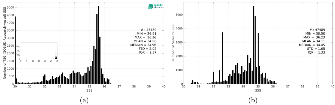
Figure 3: Histograms of SSS from TSG (GOSUD-Research-vessel) (a) and SMOS SSS L4 v1 - Monthly (CMEMS-CNR) (b) considering all match-up pairs per bins of 0.1 over the Congo river plume Pi-MEP region and for the full satellite product period.
