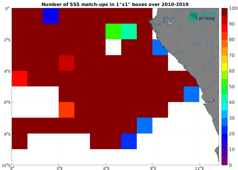
Figure 5: Number of SSS match-ups between TSG (GOSUD-Research-vessel) SSS and the SMOS SSS L4 v1 - Monthly (CMEMS-CNR) SSS product for the Congo river plume Pi-MEP region over 1^\circ \times 1^\circ boxes and for the full satellite product period.
