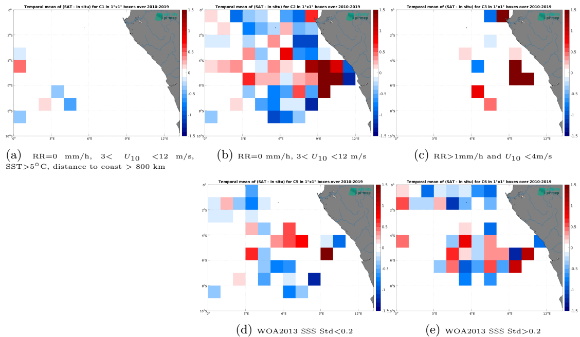
Figure 14: Temporal mean gridded over spatial boxes of size 1^\circ \times 1^\circ of \Delta SSS (SMOS SSS L4 v1 - Monthly (CMEMS-CNR) - TSG (GOSUD-Research-vessel)) for 5 different subdatasets corresponding to:RR=0 mm/h, 3 < U_{10} < 12 m/s, SST>5°C, distance to coast > 800 km (a), RR=0 mm/h, 3 < U_{10} < 12 m/s (b), RR>1mm/h and U_{10} < 4 m/s (c), WOA2013 SSS Std<0.2 (d), WOA2013 SSS Std>0.2 (e).
