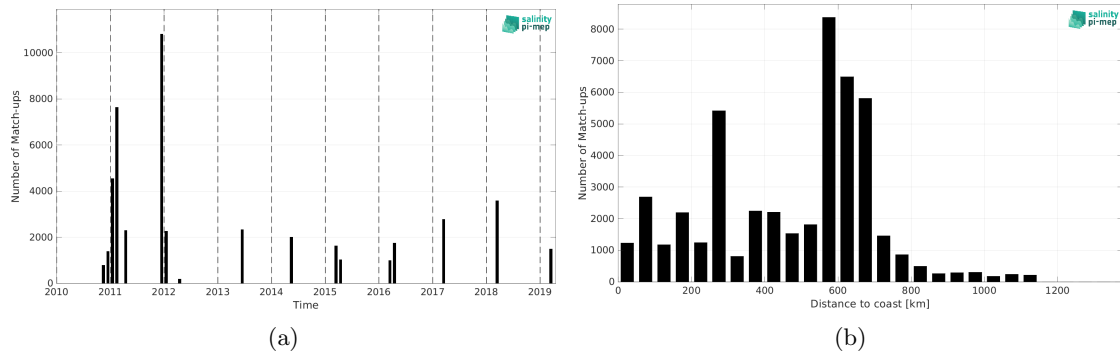
Figure 2: Number of match-ups between TSG (GOSUD-Research-vessel) and SMOS SSS L4 v1 - Monthly (CMEMS-CNR) SSS as a function of time (a) and as function of the distance to coast (b) over the Congo river plume Pi-MEP region and for the full satellite product period.
