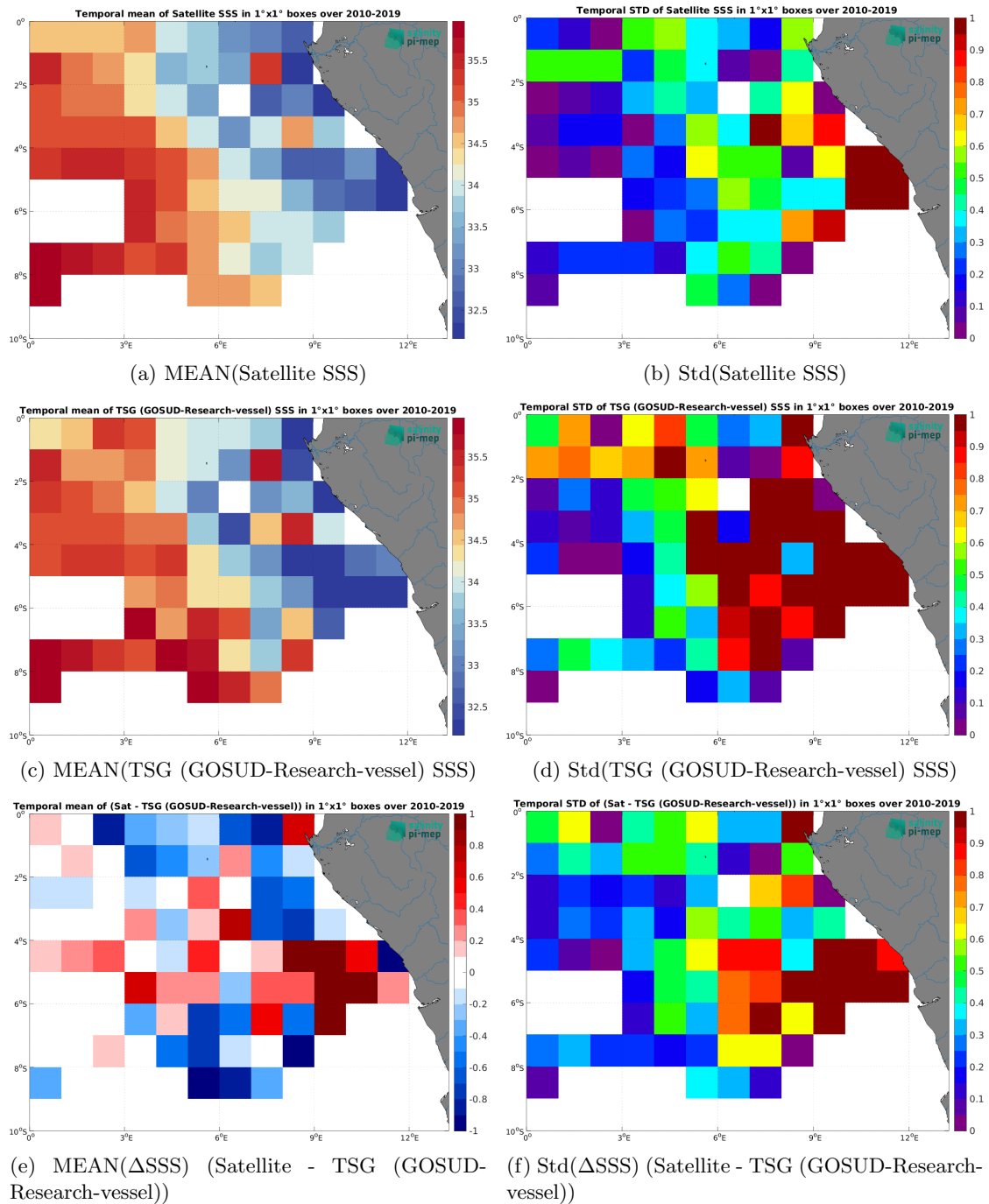
Figure 7: Temporal mean (left) and Std (right) of SSS from SMOS SSS L4 v1 - Monthly (CMEMS-CNR) (top), TSG (GOSUD-Research-vessel) (middle), and of \Delta SSS (Satellite - TSG (GOSUD-Research-vessel)). Only match-up pairs are used to generate these maps.
