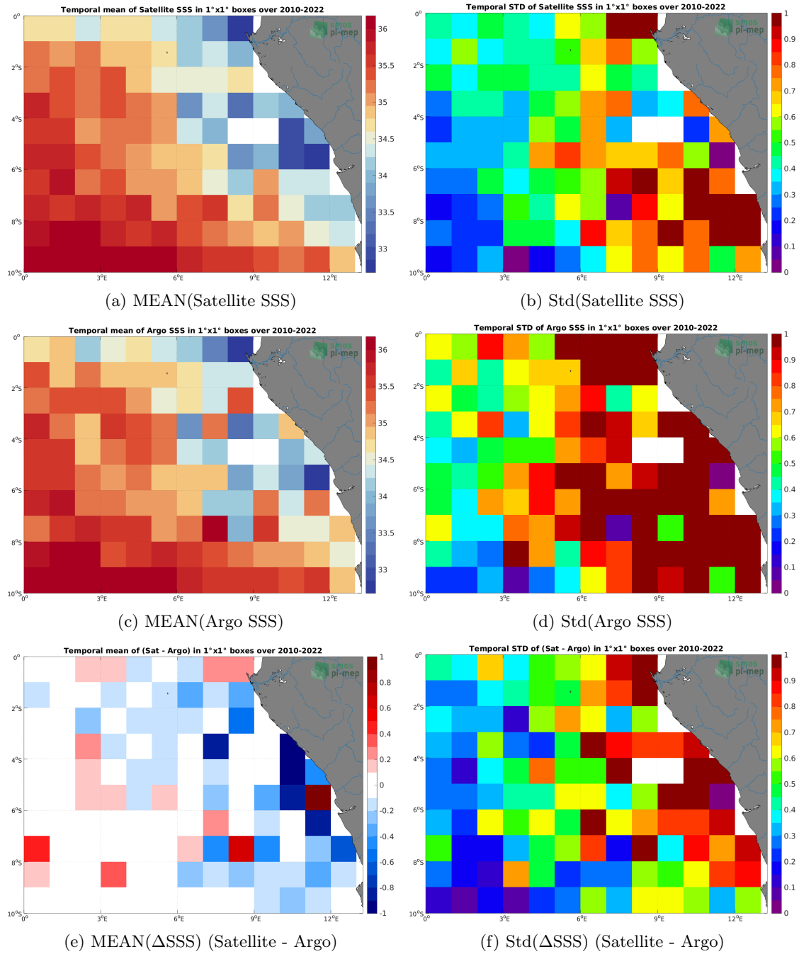
Figure 6: Temporal mean (left) and Std (right) of SSS from SMOS SSS L4 v1 - Monthly (CMEMS-CNR) (top), Argo (middle), and of \Delta SSS (Satellite - Argo). Only match-up pairs are used to generate these maps.
