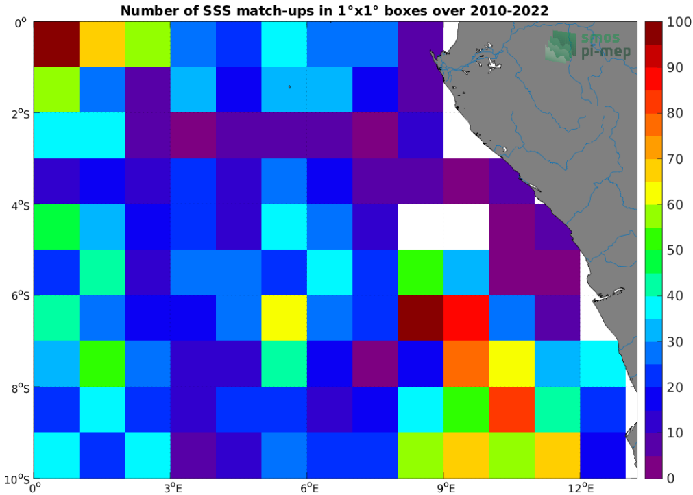
Figure 4: Number of SSS match-ups between Argo SSS and the SMOS SSS L4 v1 - Monthly (CMEMS-CNR) SSS product for the Congo river plume Pi-MEP region over 1°x1° boxes and for the full satellite product period.
