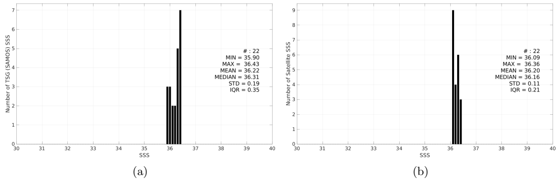
Figure 3: Histograms of SSS from TSG (SAMOS) (a) and SMOS SSS L4 v1 - Daily (CMEMS-CNR) (b) considering all match-up pairs per bins of 0.1 over the Congo river plume Pi-MEP region and for the full satellite product period.
