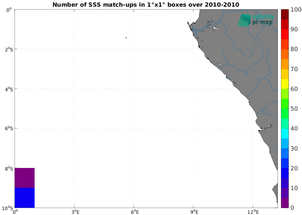
Figure 5: Number of SSS match-ups between TSG (SAMOS) SSS and the SMOS SSS L4 v1 - Daily (CMEMS-CNR) SSS product for the Congo river plume Pi-MEP region over 1^\circ \times 1^\circ boxes and for the full satellite product period.
