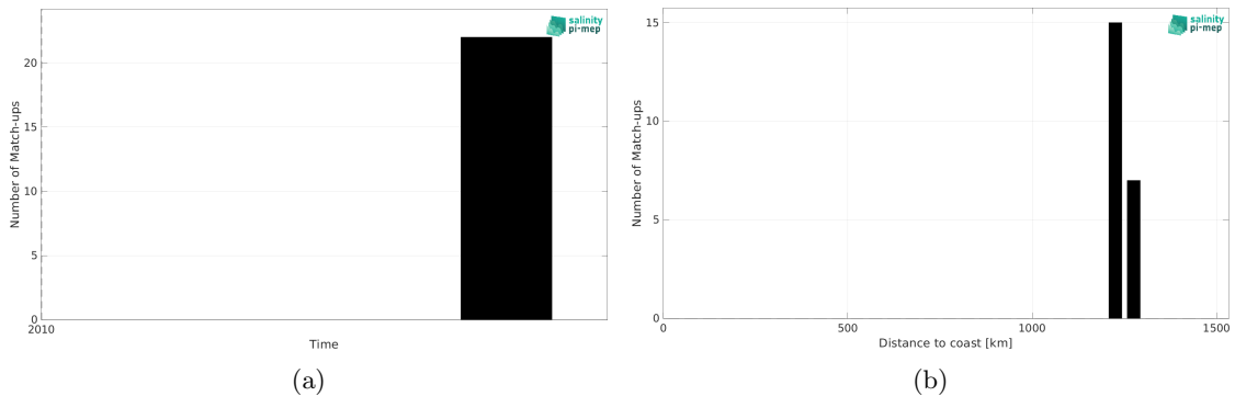
Figure 2: Number of match-ups between TSG (SAMOS) and SMOS SSS L4 v1 - Daily (CMEMS-CNR) SSS as a function of time (a) and as function of the distance to coast (b) over the Congo river plume Pi-MEP region and for the full satellite product period.
