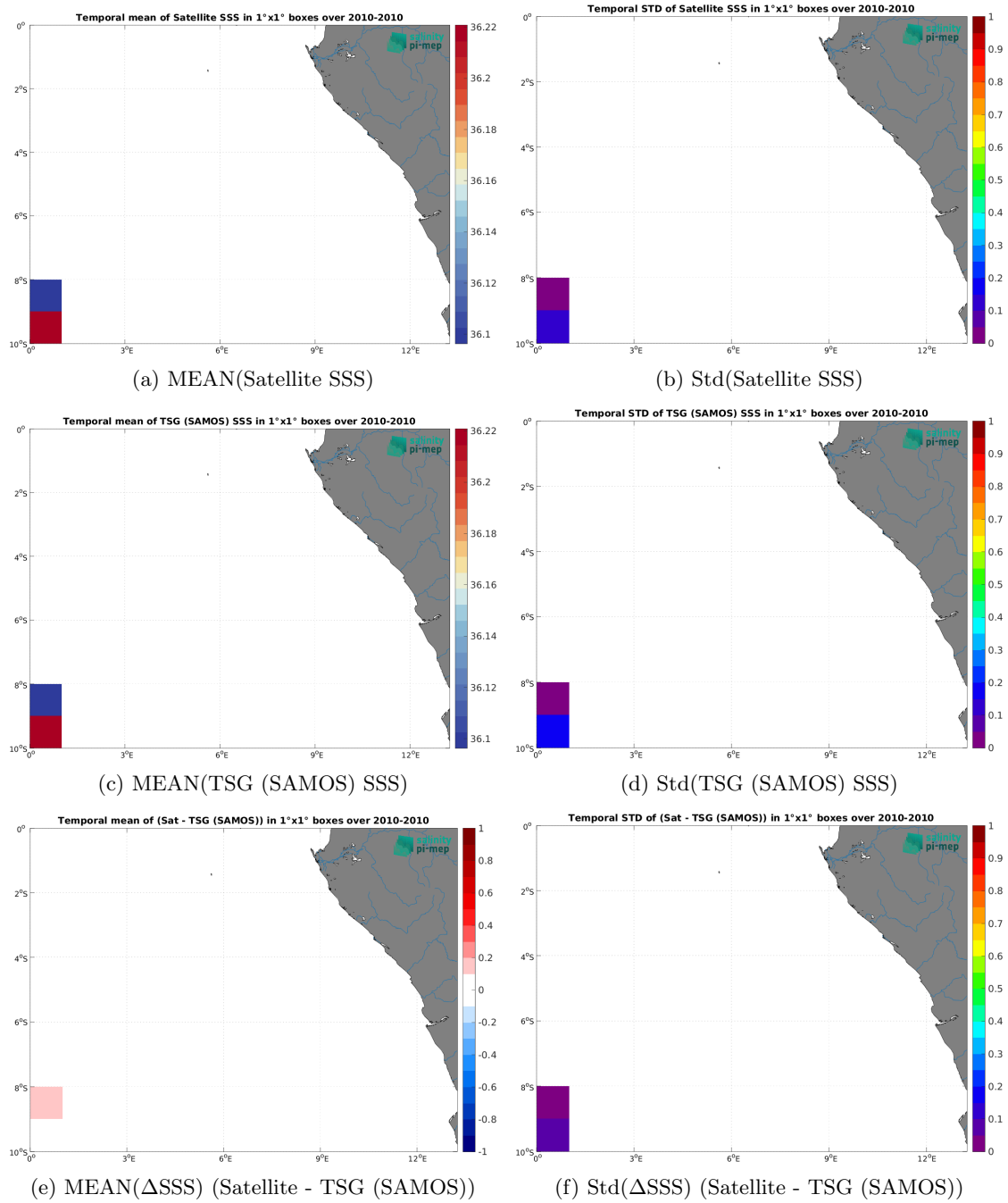
Figure 7: Temporal mean (left) and Std (right) of SSS from SMOS SSS L4 v1 - Daily (CMEMS-CNR) (top), TSG (SAMOS) (middle), and of \Delta SSS (Satellite - TSG (SAMOS)). Only match-up pairs are used to generate these maps.
