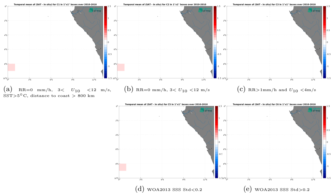
Figure 14: Temporal mean gridded over spatial boxes of size 1^\circ \times 1^\circ of \Delta SSS (SMOS SSS L4 v1 - Daily (CMEMS-CNR) - TSG (SAMOS)) for 5 different subdatasets corresponding to: RR=0 mm/h, 3 < U_{10} < 12 m/s, SST > 5°C, distance to coast > 800 km (a), RR=0 mm/h, 3 < U_{10} < 12 m/s (b), RR > 1mm/h and U_{10} < 4 m/s (c), WOA2013 SSS Std < 0.2 (d), WOA2013 SSS Std > 0.2 (e).
