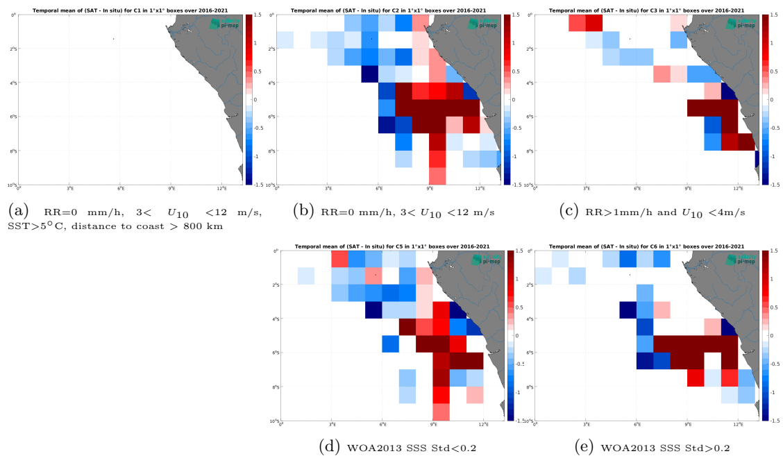
Figure 14: Temporal mean gridded over spatial boxes of size 1^\circ \times 1^\circ of \Delta SSS (SMOS SSS L4 v1 - Daily (CMEMS-CNR) - TSG (LEGOS-DM)) for 5 different subdatasets corresponding to: RR=0 mm/h, 3 < U_{10} < 12 m/s, SST > 5°C, distance to coast > 800 km (a), RR=0 mm/h, 3 < U_{10} < 12 m/s (b), RR > 1mm/h and U_{10} < 4 m/s (c), WOA2013 SSS Std < 0.2 (d), WOA2013 SSS Std > 0.2 (e).
