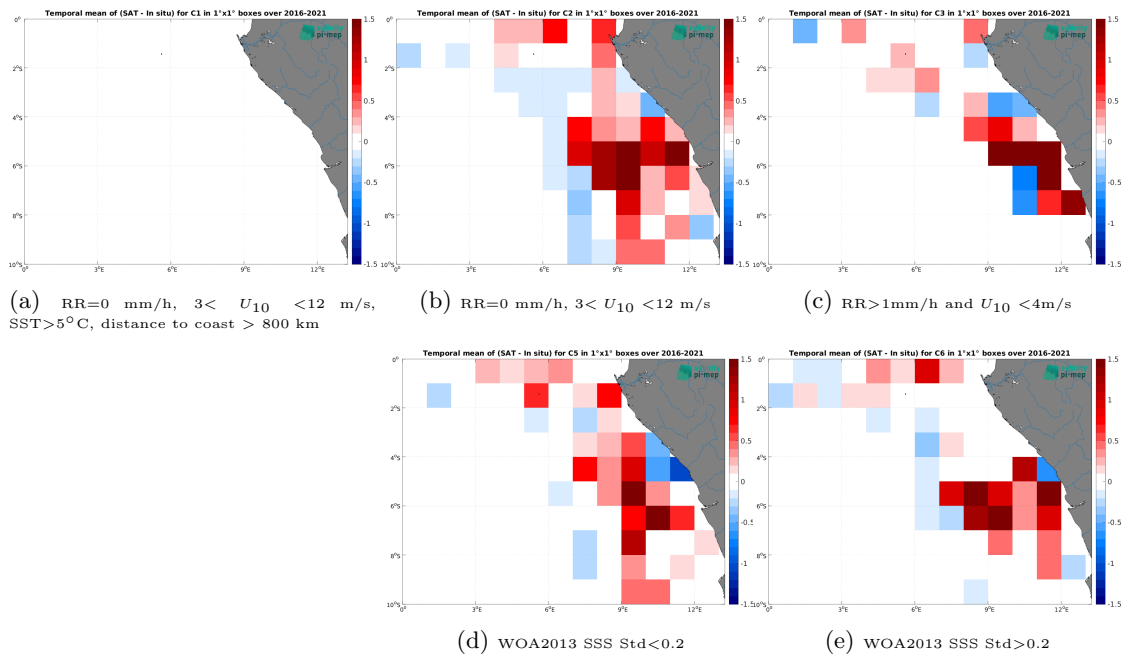
Figure 14: Temporal mean gridded over spatial boxes of size 1^\circ \times 1^\circ of \Delta SSS (SMOS SSS L4 OI v346 - Weekly (CMEMS-CATDS-LOPS) - TSG (LEGOS-DM)) for 5 different subdatasets corresponding to:RR=0 mm/h, 3 < U_{10} < 12 m/s, SST>5°C, distance to coast > 800 km (a), RR=0 mm/h, 3 < U_{10} < 12 m/s (b), RR>1mm/h and U_{10} < 4 m/s (c), WOA2013 SSS Std<0.2 (d), WOA2013 SSS Std>0.2 (e).
