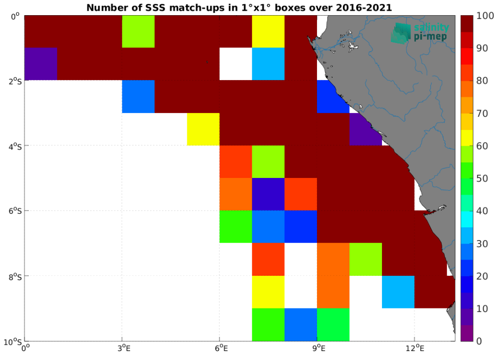
Figure 5: Number of SSS match-ups between TSG (LEGOS-DM) SSS and the SMOS SSS L4 OI v346 - Weekly (CMEMS-CATDS-LOPS) SSS product for the Congo river plume Pi-MEP region over 1^\circ \times 1^\circ boxes and for the full satellite product period.
