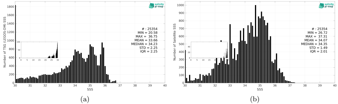
Figure 3: Histograms of SSS from TSG (LEGOS-DM) (a) and SMOS SSS L4 OI v346 - Weekly (CMEMS-CATDS-LOPS) (b) considering all match-up pairs per bins of 0.1 over the Congo river plume Pi-MEP region and for the full satellite product period.
