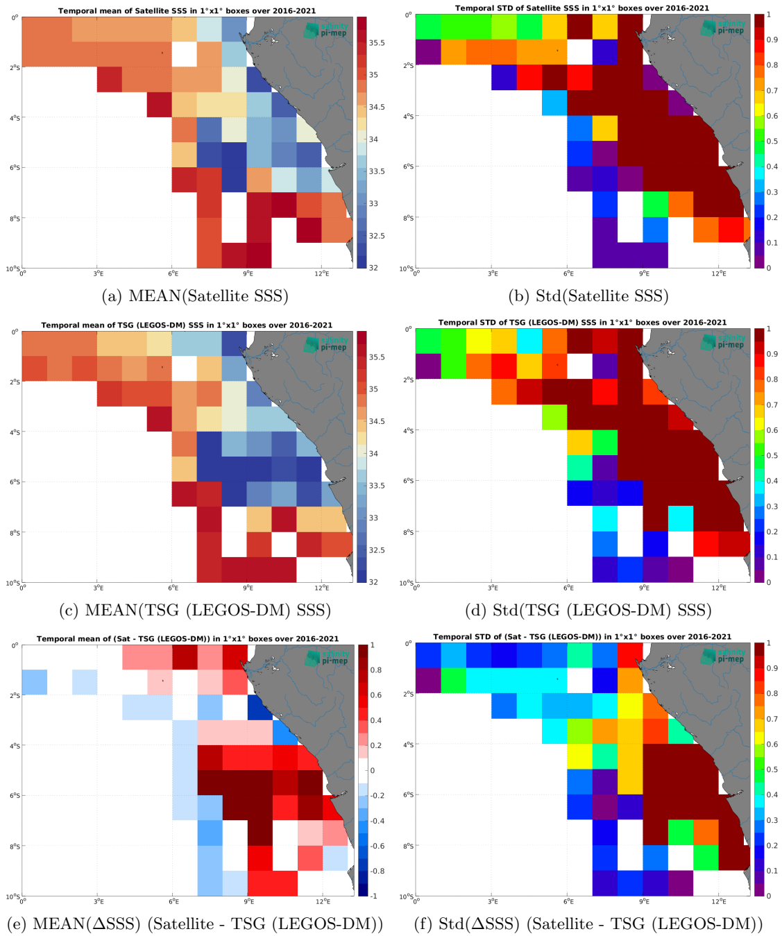
Figure 7: Temporal mean (left) and Std (right) of SSS from SMOS SSS L4 OI v346 - Weekly (CMEMS-CATDS-LOPS) (top), TSG (LEGOS-DM) (middle), and of \Delta SSS (Satellite - TSG (LEGOS-DM)). Only match-up pairs are used to generate these maps.
