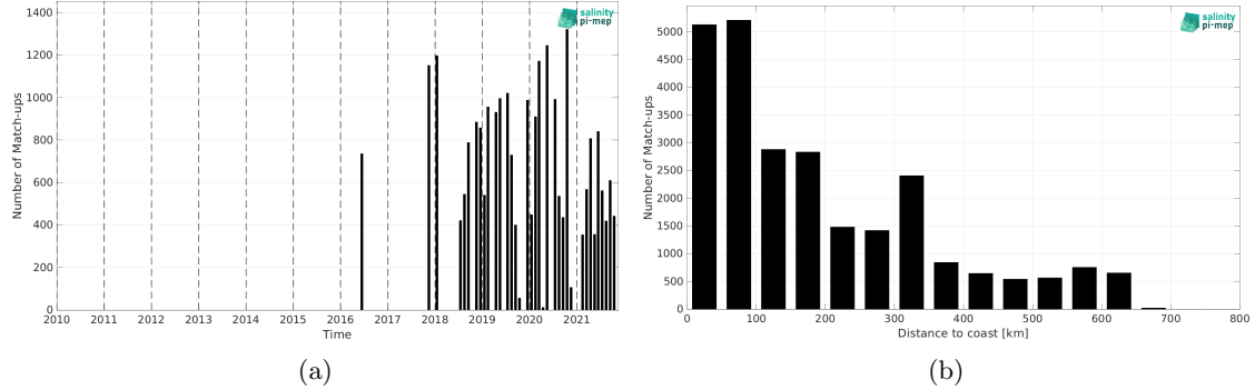
Figure 2: Number of match-ups between TSG (LEGOS-DM) and SMOS SSS L4 OI v346 - Weekly (CMEMS-CATDS-LOPS) SSS as a function of time (a) and as function of the distance to coast (b) over the Congo river plume Pi-MEP region and for the full satellite product period.
