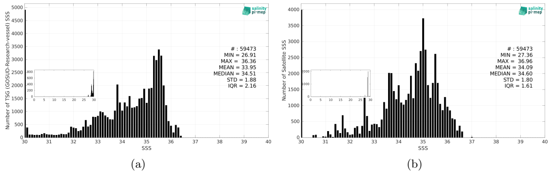
Figure 3: Histograms of SSS from TSG (GOSUD-Research-vessel) (a) and SMOS SSS L4 OI v346 - Weekly (CMEMS-CATDS-LOPS) (b) considering all match-up pairs per bins of 0.1 over the Congo river plume Pi-MEP region and for the full satellite product period.
