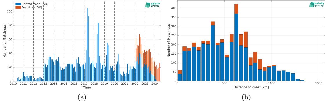
Figure 2: Number of match-ups between Argo and SMOS SSS L4 OI v346 - Weekly (CMEMS-CATDS-LOPS) SSS as a function of time (a) and as function of the distance to coast (b) over the Congo river plume Pi-MEP region and for the full satellite product period.
