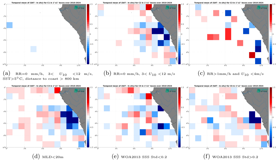
Figure 14: Temporal mean gridded over spatial boxes of size 1^\circ \times 1^\circ of \Delta SSS (SMOS SSS L4 OI v346 - Weekly (CMEMS-CATDS-LOPS) - Argo) for 6 different subdatasets corresponding to:RR=0 mm/h, 3 < U_{10} < 12 m/s, SST>5°C, distance to coast > 800 km (a), RR=0 mm/h, 3 < U_{10} < 12 m/s (b), RR>1mm/h and U_{10} < 4 m/s (c),MLD<20m (d),WOA2013 SSS Std<0.2 (e),WOA2013 SSS Std>0.2 (f).
