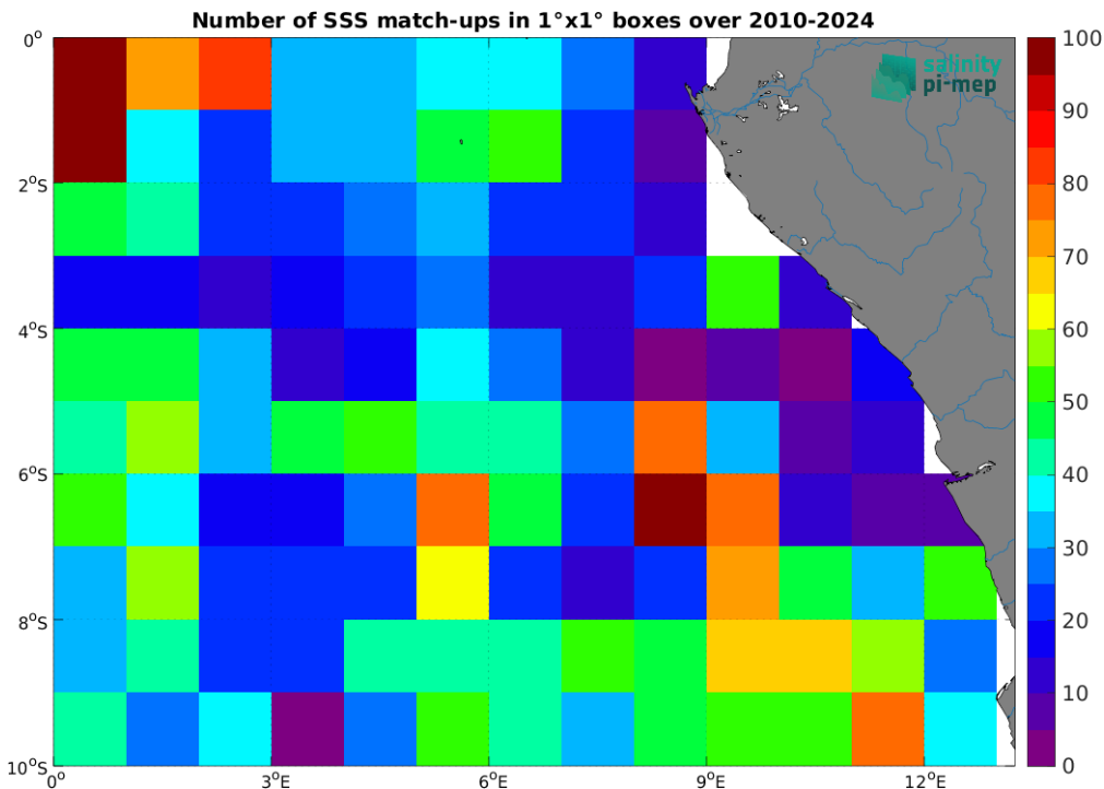
Figure 5: Number of SSS match-ups between Argo SSS and the SMOS SSS L4 OI v346 - Weekly (CMEMS-CATDS-LOPS) SSS product for the Congo river plume Pi-MEP region over 1^\circ \times 1^\circ boxes and for the full satellite product period.
