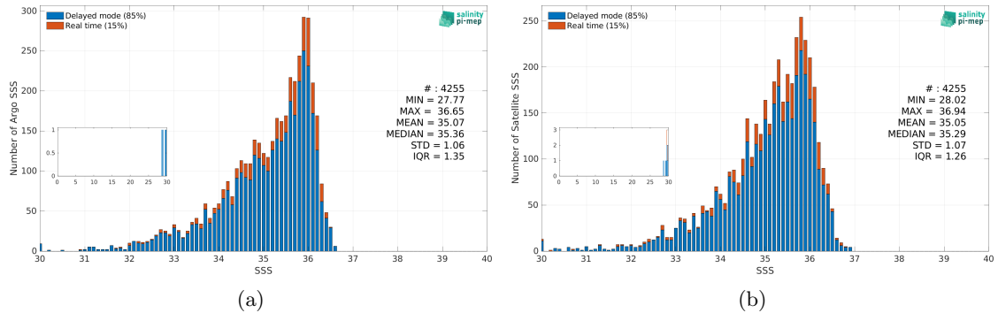
Figure 3: Histograms of SSS from Argo (a) and SMOS SSS L4 OI v346 - Weekly (CMEMS-CATDS-LOPS) (b) considering all match-up pairs per bins of 0.1 over the Congo river plume Pi-MEP region and for the full satellite product period.
