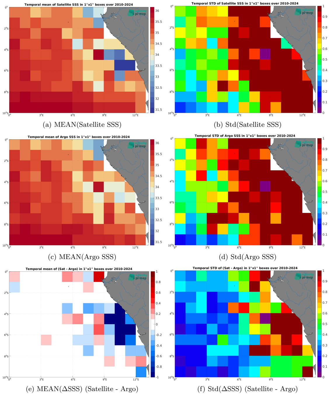
Figure 7: Temporal mean (left) and Std (right) of SSS from SMOS SSS L4 OI v346 - Weekly (CMEMS-CATDS-LOPS) (top), Argo (middle), and of \Delta SSS (Satellite - Argo). Only match-up pairs are used to generate these maps.
