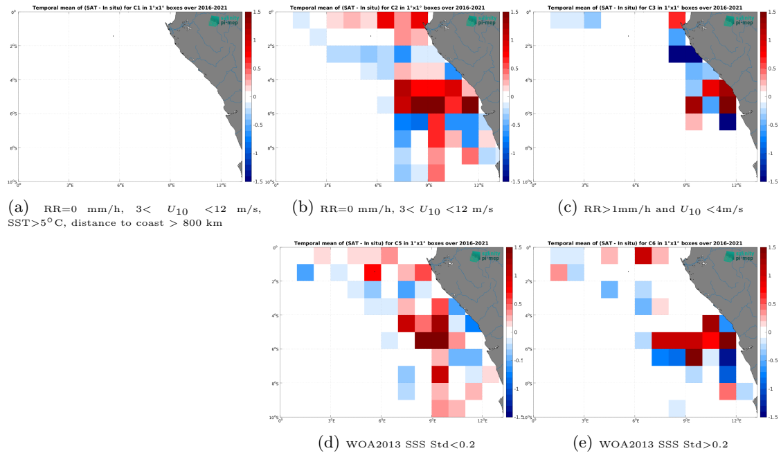
Figure 12: Temporal mean gridded over spatial boxes of size 1^{\circ}\times 1^{\circ} of \Delta\text{SSS} (SMOS SSS L4 OI v342 - Weekly (CMEMS-CATDS-LOPS) - TSG (LEGOS-DM)) for 5 different subdatasets corresponding to:RR=0 mm/h, 3 < U_{10} < 12 m/s, SST >5^{\circ}\text{C} , distance to coast > 800 km (a), RR=0 mm/h, 3 < U_{10} < 12 m/s (b), RR >1 mm/h and U_{10} < 4 m/s (c), WOA2013 SSS Std <0.2 (d), WOA2013 SSS Std >0.2 (e).
