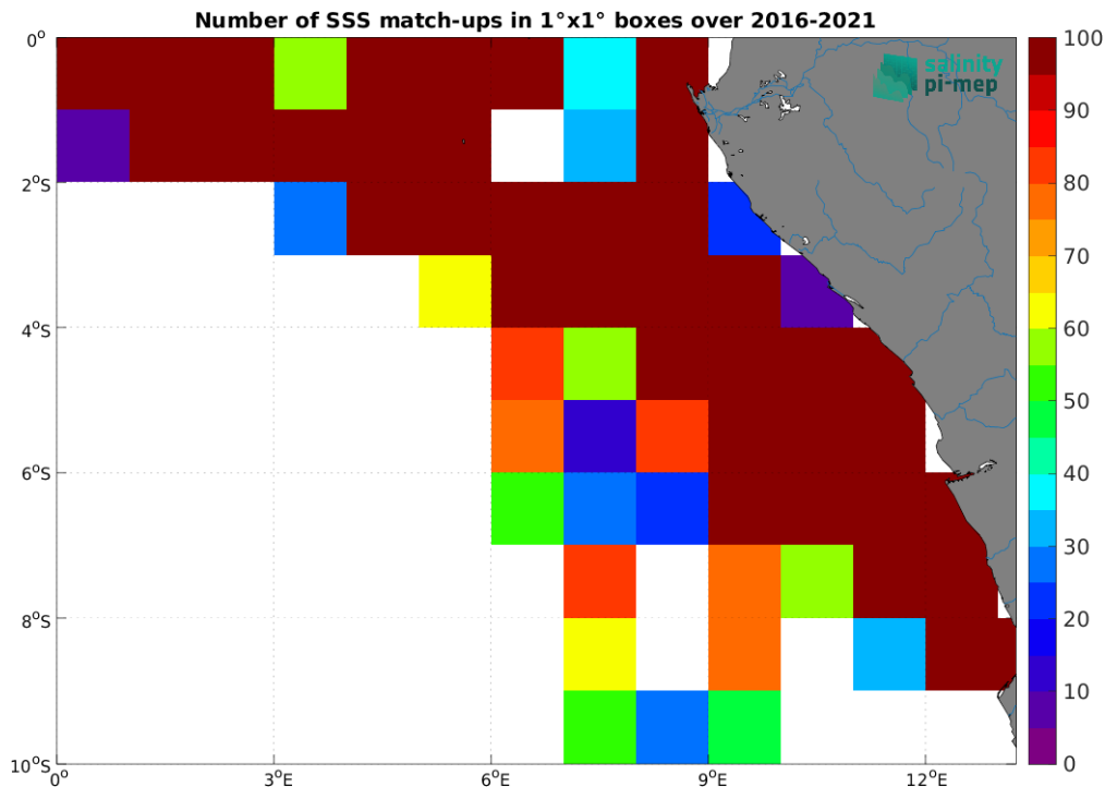
Figure 4: Number of SSS match-ups between TSG (LEGOS-DM) SSS and the SMOS SSS L4 OI v342 - Weekly (CMEMS-CATDS-LOPS) SSS product for the Congo river plume Pi-MEP region over 1^\circ \times 1^\circ boxes and for the full satellite product period.
