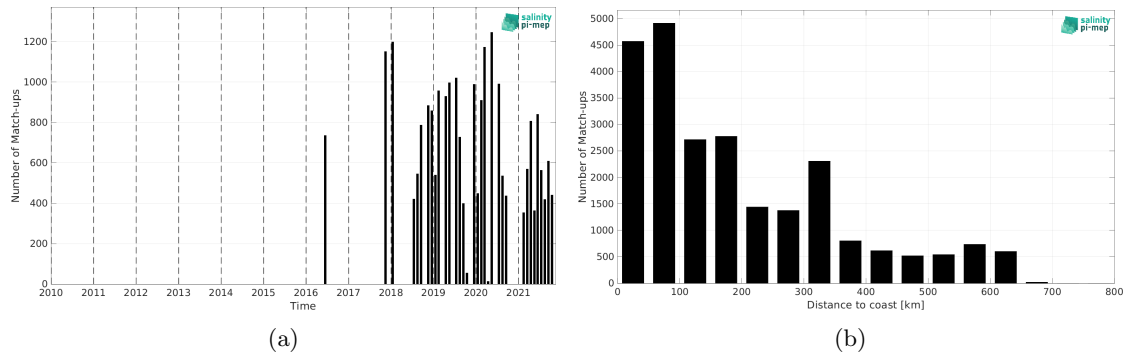
Figure 1: Number of match-ups between TSG (LEGOS-DM) and SMOS SSS L4 OI v342 - Weekly (CMEMS-CATDS-LOPS) SSS as a function of time (a) and as function of the distance to coast (b) over the Congo river plume Pi-MEP region and for the full satellite product period.
