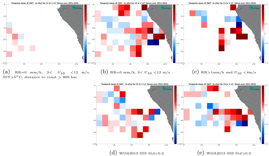
Figure 12: Temporal mean gridded over spatial boxes of size 1^\circ \times 1^\circ of \Delta\text{SSS} (SMOS SSS L4 OI v342 - Weekly (CMEMS-CATDS-LOPS) - TSG (GOSUD-Research-vessel)) for 5 different subdatasets corresponding to:RR=0 mm/h, 3 < U_{10} < 12 m/s, SST > 5^\circ\text{C} , distance to coast > 800 km (a), RR=0 mm/h, 3 < U_{10} < 12 m/s (b), RR > 1 mm/h and U_{10} < 4 m/s (c), WOA2013 SSS Std < 0.2 (d), WOA2013 SSS Std > 0.2 (e).
