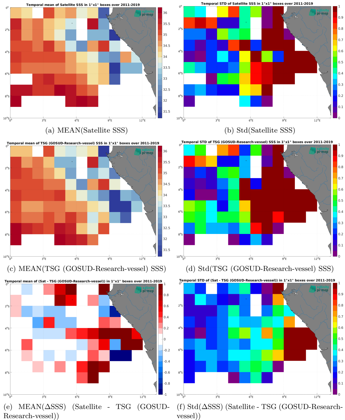
Figure 6: Temporal mean (left) and Std (right) of SSS from SMOS SSS L4 OI v342 - Weekly (CMEMS-CATDS-LOPS) (top), TSG (GOSUD-Research-vessel) (middle), and of \Delta SSS (Satellite - TSG (GOSUD-Research-vessel)). Only match-up pairs are used to generate these maps.
