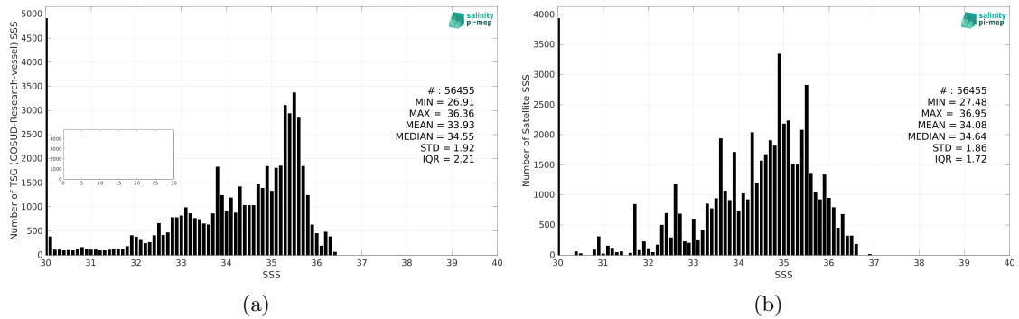
Figure 2: Histograms of SSS from TSG (GOSUD-Research-vessel) (a) and SMOS SSS L4 OI v342 - Weekly (CMEMS-CATDS-LOPS) (b) considering all match-up pairs per bins of 0.1 over the Congo river plume Pi-MEP region and for the full satellite product period.
