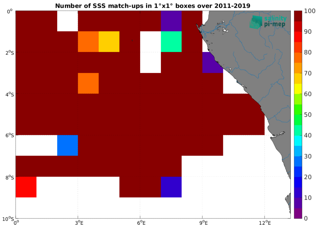
Figure 4: Number of SSS match-ups between TSG (GOSUD-Research-vessel) SSS and the SMOS SSS L4 OI v342 - Weekly (CMEMS-CATDS-LOPS) SSS product for the Congo river plume Pi-MEP region over 1^\circ \times 1^\circ boxes and for the full satellite product period.
