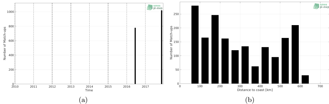
Figure 1: Number of match-ups between TSG (LEGOS-DM) and SMOS L4 v2 Weekly (CATDS-CECOS-IFREMER) SSS as a function of time (a) and as function of the distance to coast (b) over the Congo river plume Pi-MEP region and for the full satellite product period.
