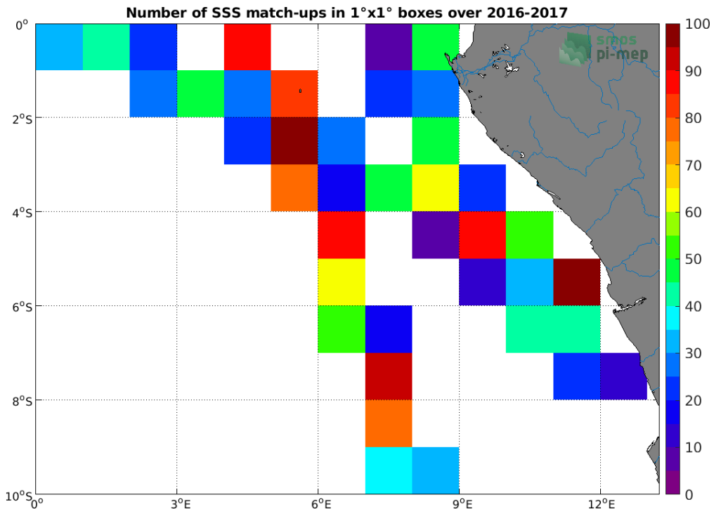
Figure 4: Number of SSS match-ups between TSG (LEGOS-DM) SSS and the SMOS L4 v2 Weekly (CATDS-CECOS-IFREMER) SSS product for the Congo river plume Pi-MEP region over 1^\circ \times 1^\circ boxes and for the full satellite product period.
