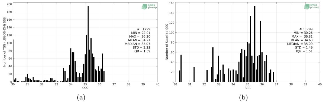
Figure 2: Histograms of SSS from TSG (LEGOS-DM) (a) and SMOS L4 v2 Weekly (CATDS-CECOS-IFREMER) (b) considering all match-up pairs per bins of 0.1 over the Congo river plume Pi-MEP region and for the full satellite product period.
