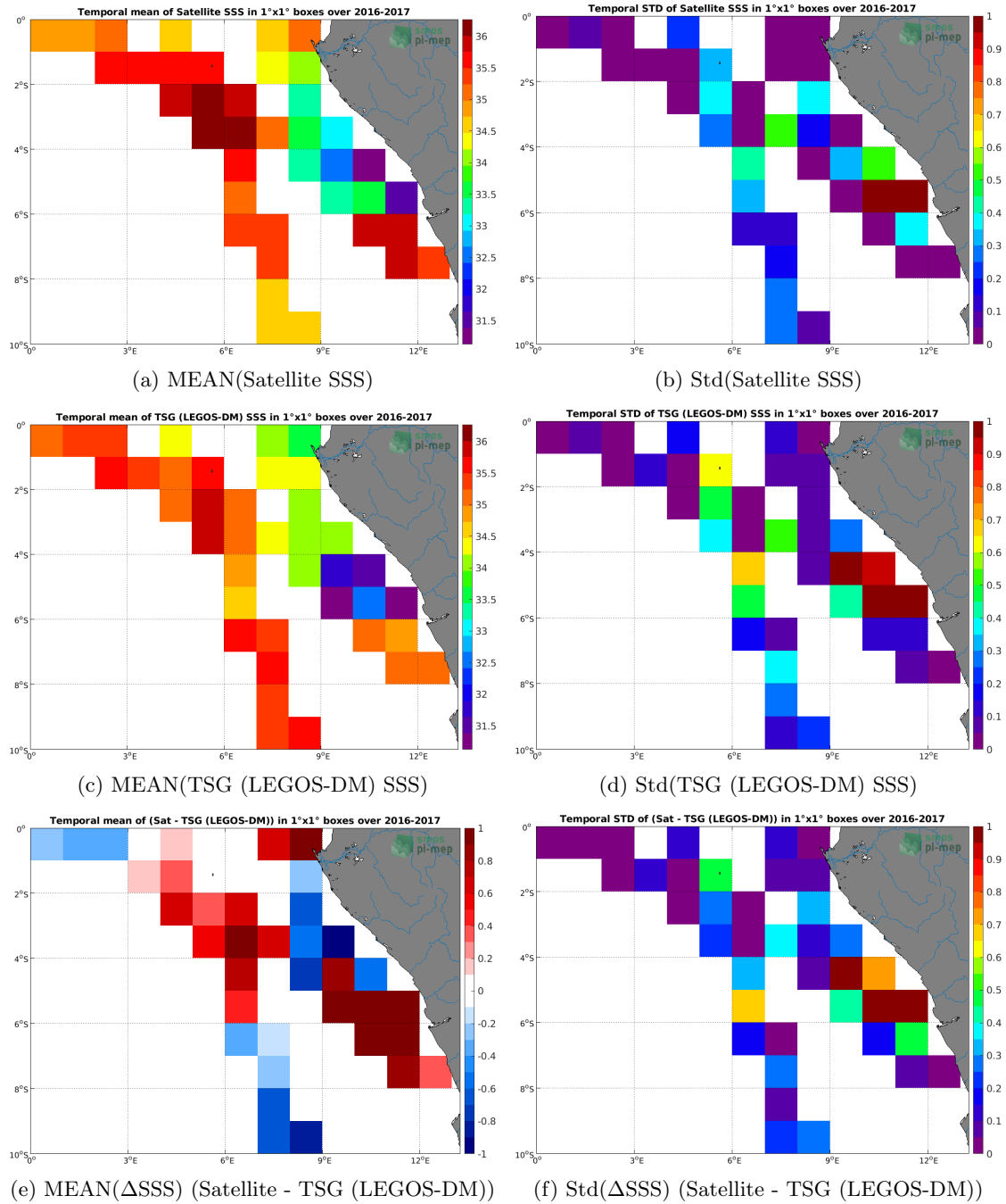
Figure 6: Temporal mean (left) and Std (right) of SSS from SMOS L4 v2 Weekly (CATDS-CECOS-IFREMER) (top), TSG (LEGOS-DM) (middle), and of \Delta SSS (Satellite - TSG (LEGOS-DM)). Only match-up pairs are used to generate these maps.
