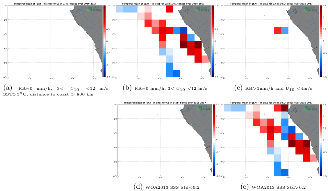
Figure 12: Temporal mean gridded over spatial boxes of size 1^{\circ}\times 1^{\circ} of \Delta\text{SSS} (SMOS L4 v2 Weekly (CATDS-CECOS-IFREMER) - TSG (LEGOS-DM)) for 5 different subdatasets corresponding to:RR=0 mm/h, 3 < U_{10} < 12 m/s, SST >5^{\circ}\text{C} , distance to coast > 800 km (a), RR=0 mm/h, 3 < U_{10} < 12 m/s (b), RR >1 mm/h and U_{10} < 4 m/s (c), WOA2013 SSS Std <0.2 (d), WOA2013 SSS Std >0.2 (e).
