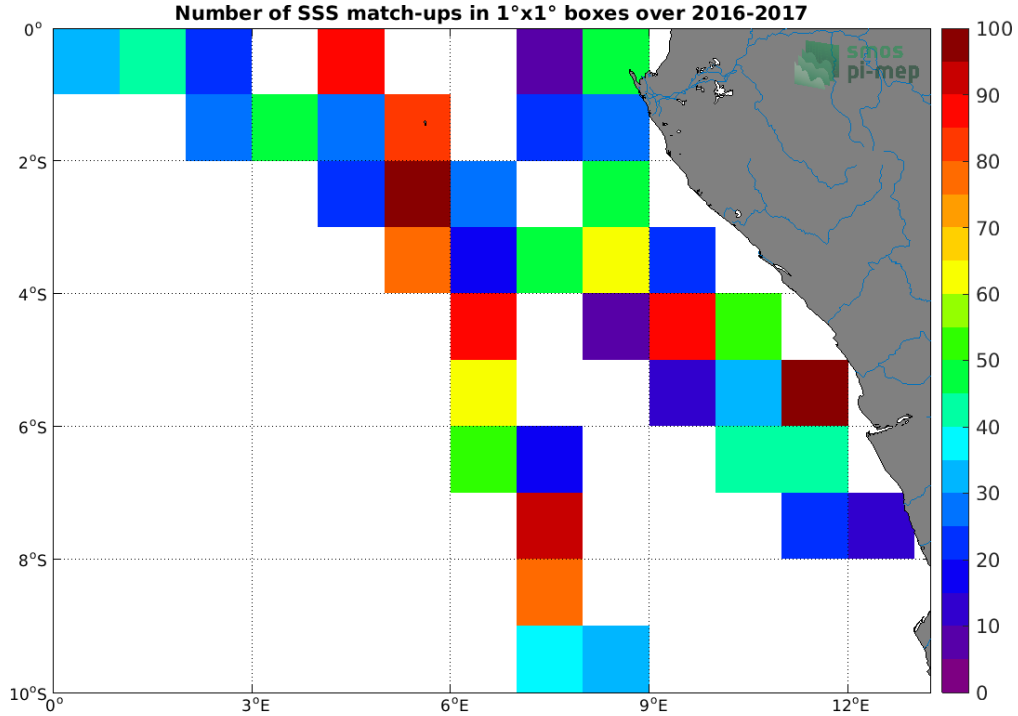
Figure 4: Number of SSS match-ups between TSG (LEGOS-DM) SSS and the SMOS L4 v2 Weekly (CATDS-CECOS-IFREMER) SSS product for the Congo river plume Pi-MEP region over 1°x1° boxes and for the full satellite product period.
