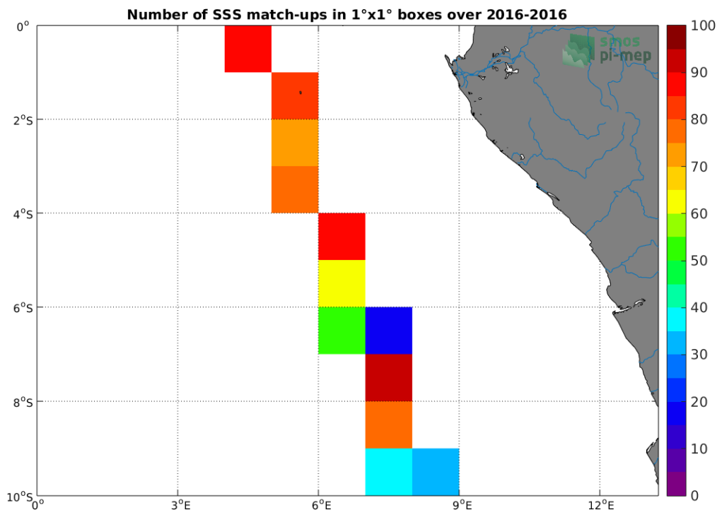
Figure 4: Number of SSS match-ups between TSG-LEGOS-DM SSS and the SMOS-L4-CATDS-CECOS-IFREMER-V2-WEEKLY-0.5DEG SSS product for the Congo river plume Pi-MEP region over 1°x1° boxes and for the full satellite product period.
