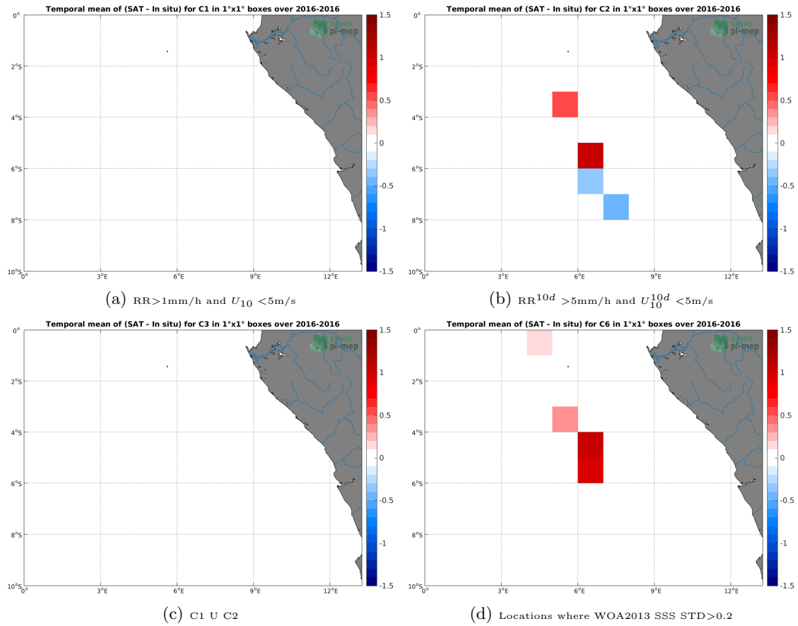
Figure 12: Temporal mean gridded over spatial boxes of size 1^\circ \times 1^\circ of \Delta SSS (SMOS-L4-CATDS-CECOS-IFREMER-V2-WEEKLY-0.5DEG - TSG-LEGOS-DM) for 4 different subdatasets corresponding to: RR > 1\text{mm/h} and U_{10} < 5\text{m/s} (a), RR^{10d} > 5\text{mm/h} and U_{10}^{10d} < 5\text{m/s} (b), C1 \cup C2 (c), Locations where WOA2013 SSS STD > 0.2 (d).
