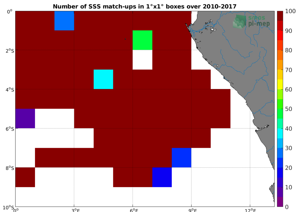
Figure 4: Number of SSS match-ups between TSG (GOSUD-Research-vessel) SSS and the SMOS L4 v2 Weekly (CATDS-CECOS-IFREMER) SSS product for the Congo river plume Pi-MEP region over 1^\circ \times 1^\circ boxes and for the full satellite product period.
