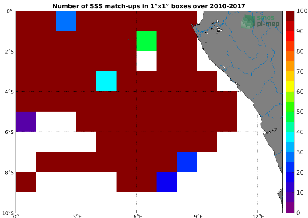
Figure 4: Number of SSS match-ups between TSG (GOSUD-Research-vessel) SSS and the SMOS L4 v2 Weekly (CATDS-CECOS-IFREMER) SSS product for the Congo river plume Pi-MEP region over 1°x1° boxes and for the full satellite product period.
