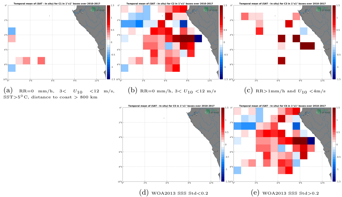
Figure 12: Temporal mean gridded over spatial boxes of size 1^\circ \times 1^\circ of \Delta SSS (SMOS L4 v2 Weekly (CATDS-CECOS-IFREMER) - TSG (GOSUD-Research-vessel)) for 5 different subdatasets corresponding to: RR=0 mm/h, 3 < U_{10} < 12 m/s, SST > 5^\circ\text{C} , distance to coast > 800 km (a), RR=0 mm/h, 3 < U_{10} < 12 m/s (b), RR > 1 mm/h and U_{10} < 4 m/s (c), WOA2013 SSS Std < 0.2 (d), WOA2013 SSS Std > 0.2 (e).
