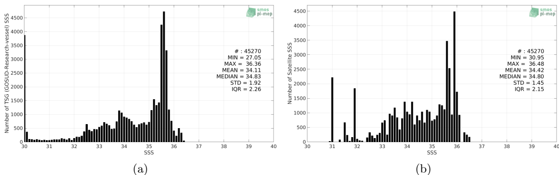
Figure 2: Histograms of SSS from TSG (GOSUD-Research-vessel) (a) and SMOS L4 v2 Weekly (CATDS-CECOS-IFREMER) (b) considering all match-up pairs per bins of 0.1 over the Congo river plume Pi-MEP region and for the full satellite product period.
