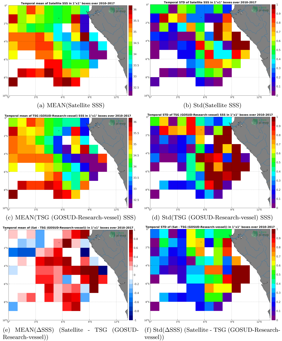
Figure 6: Temporal mean (left) and Std (right) of SSS from SMOS L4 v2 Weekly (CATDS-CECOS-IFREMER) (top), TSG (GOSUD-Research-vessel) (middle), and of \Delta SSS (Satellite - TSG (GOSUD-Research-vessel)). Only match-up pairs are used to generate these maps.
