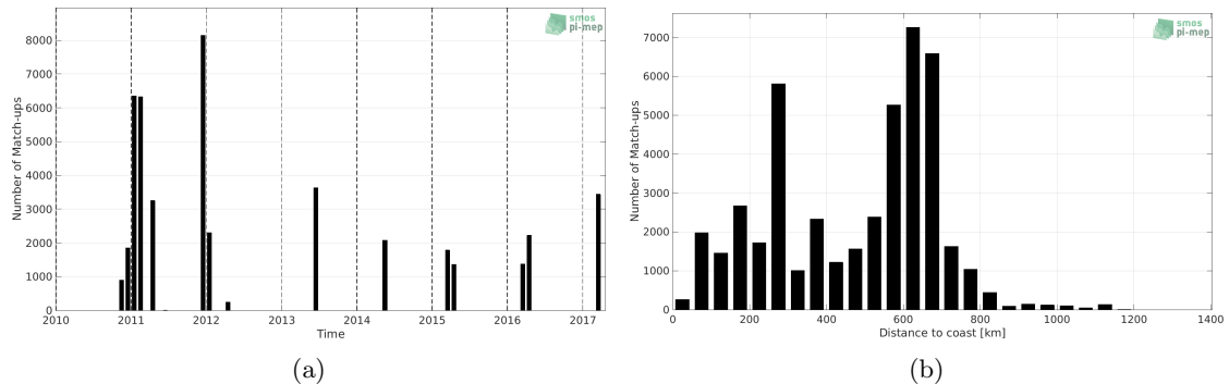
Figure 1: Number of match-ups between TSG (GOSUD-Research-vessel) and SMOS L4 v2 Weekly (CATDS-CECOS-IFREMER) SSS as a function of time (a) and as function of the distance to coast (b) over the Congo river plume Pi-MEP region and for the full satellite product period.
