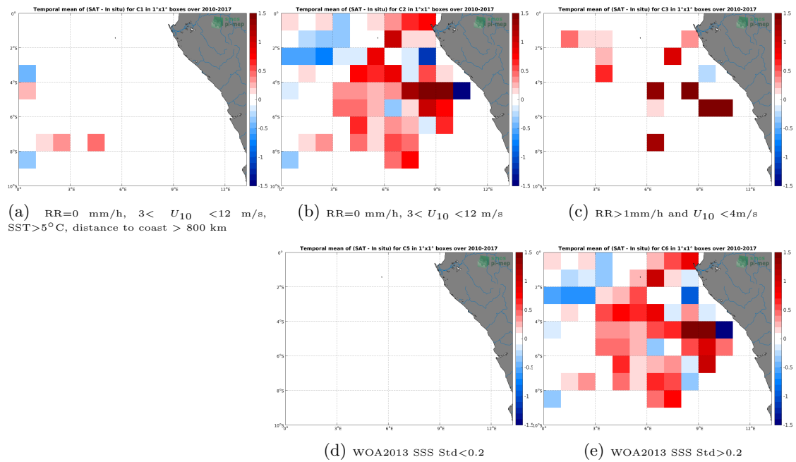
Figure 12: Temporal mean gridded over spatial boxes of size 1^\circ \times 1^\circ of \Delta SSS (SMOS-L4-CATDS-CECOS-IFREMER-V2-WEEKLY-0.5DEG - TSG-GOSUD-Research-vessel) for 5 different sub-datasets corresponding to: RR=0 mm/h, 3 < U_{10} < 12 m/s, SST > 5^\circ\text{C} , distance to coast > 800 km (a), RR=0 mm/h, 3 < U_{10} < 12 m/s (b), RR > 1 mm/h and U_{10} < 4 m/s (c), WOA2013 SSS Std < 0.2 (d), WOA2013 SSS Std > 0.2 (e).
