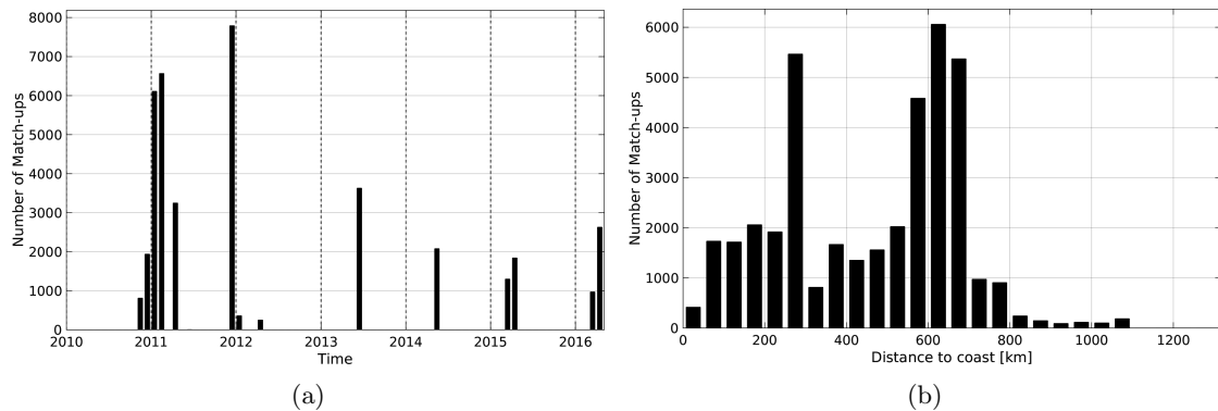
Figure 1: Number of match-ups between TSG-GOSUD-Research-vessel and SMOS-L4-CATDS-CECOS-IFREMER-V2-WEEKLY-0.5DEG SSS as a function of time (a) and as function of the distance to coast (b) over the Congo river plume Pi-MEP region and for the full satellite product period.
