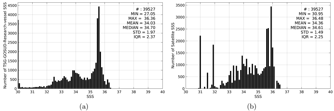
Figure 2: Histograms of SSS from TSG-GOSUD-Research-vessel (a) and SMOS-L4-CATDS-CECOS-IFREMER-V2-WEEKLY-0.5DEG (b) considering all match-up pairs per bins of 0.1 over the Congo river plume Pi-MEP region and for the full satellite product period.
