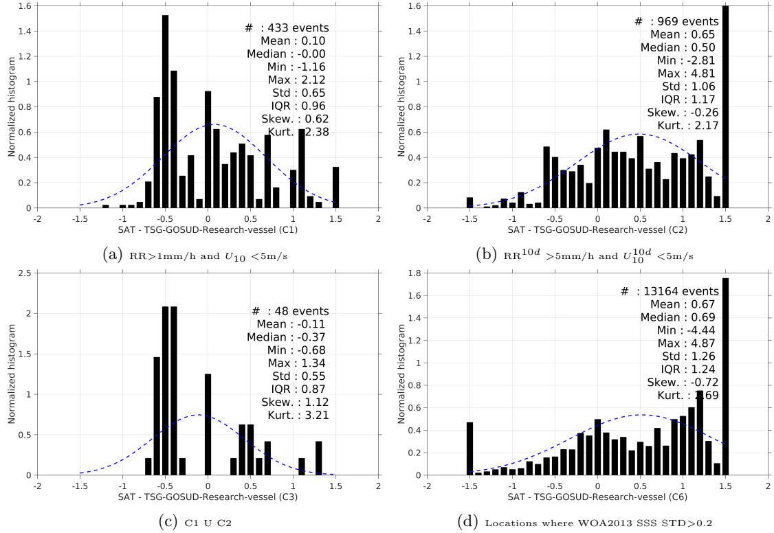
Figure 13: Normalized histogram of \Delta\text{SSS} (SMOS-L4-CATDS-CECOS-IFREMER-V2-WEEKLY-0.5DEG - TSG-GOSUD-Research-vessel) for 6 different subdatasets corresponding to: \text{RR} > 1\text{mm/h} and U_{10} < 5\text{m/s} (a), \text{RR}^{10d} > 5\text{mm/h} and U_{10}^{10d} < 5\text{m/s} (b), C1 U C2 (c), Locations where WOA2013 SSS STD > 0.2 (d).
