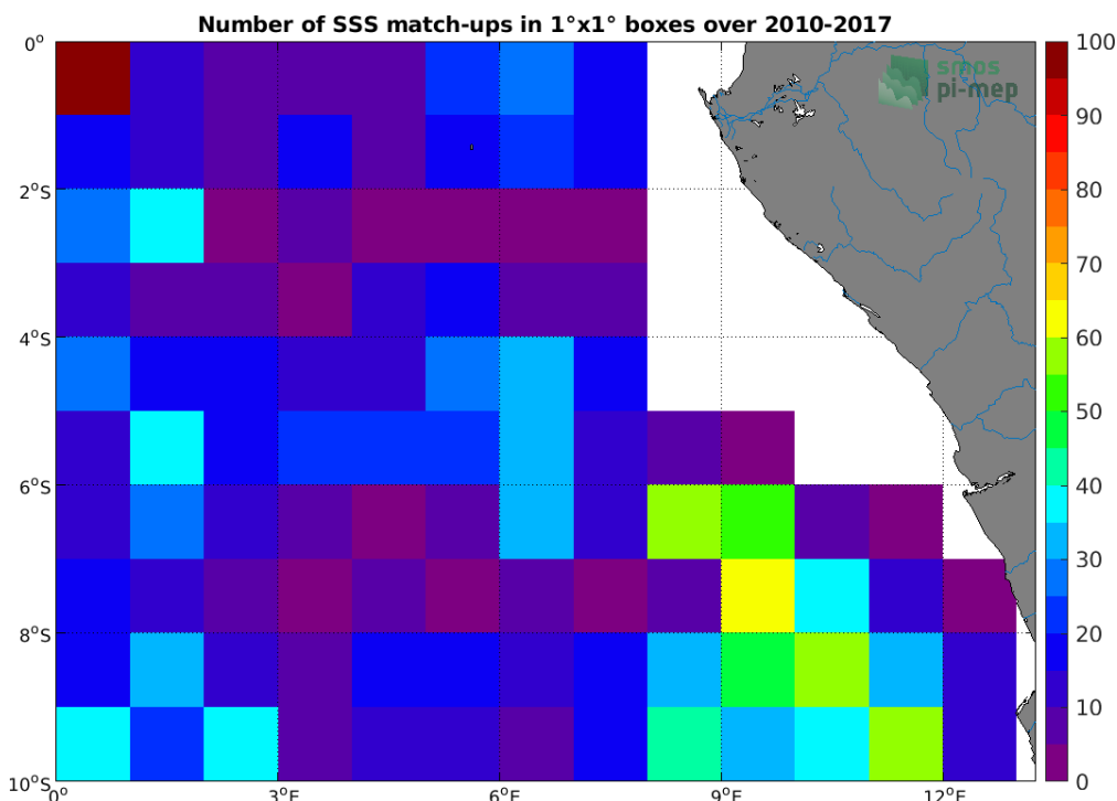
Figure 4: Number of SSS match-ups between Argo SSS and the SMOS L4 v2 Weekly (CATDS-CECOS-IFREMER) SSS product for the Congo river plume Pi-MEP region over 1^{\circ} \times 1^{\circ} boxes and for the full satellite product period.
