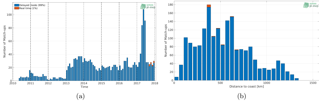
Figure 1: Number of match-ups between Argo and SMOS L4 v2 Weekly (CATDS-CECOS-IFREMER) SSS as a function of time (a) and as function of the distance to coast (b) over the Congo river plume Pi-MEP region and for the full satellite product period.
