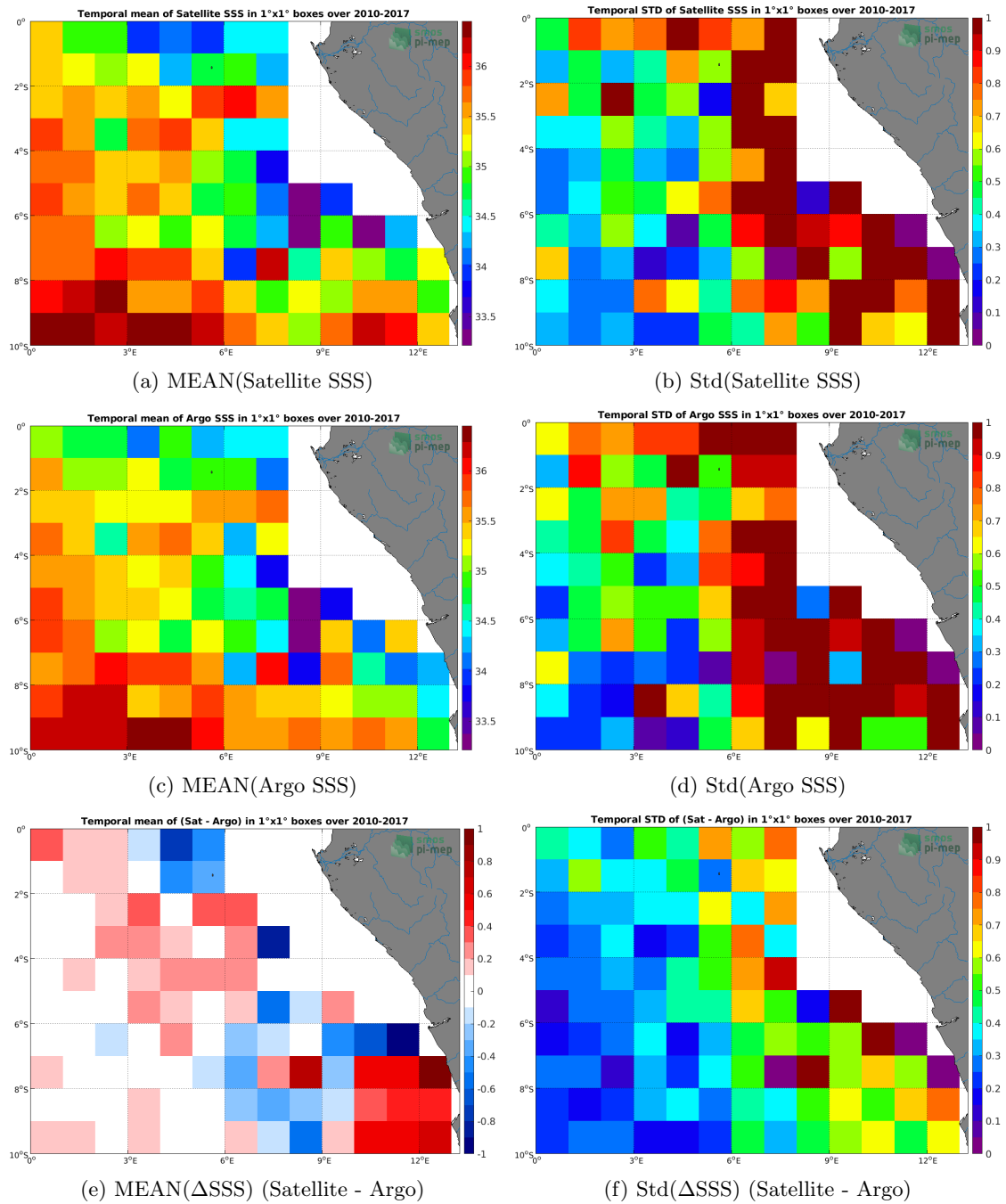
Figure 6: Temporal mean (left) and Std (right) of SSS from SMOS L4 v2 Weekly (CATDS-CECOS-IFREMER) (top), Argo (middle), and of \Delta SSS (Satellite - Argo). Only match-up pairs are used to generate these maps.
