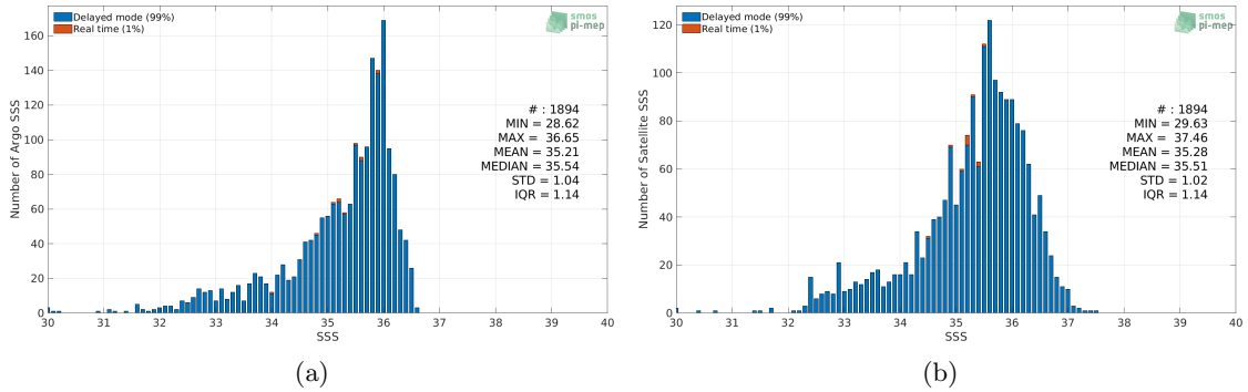
Figure 2: Histograms of SSS from Argo (a) and SMOS L4 v2 Weekly (CATDS-CECOS-IFREMER) (b) considering all match-up pairs per bins of 0.1 over the Congo river plume Pi-MEP region and for the full satellite product period.
