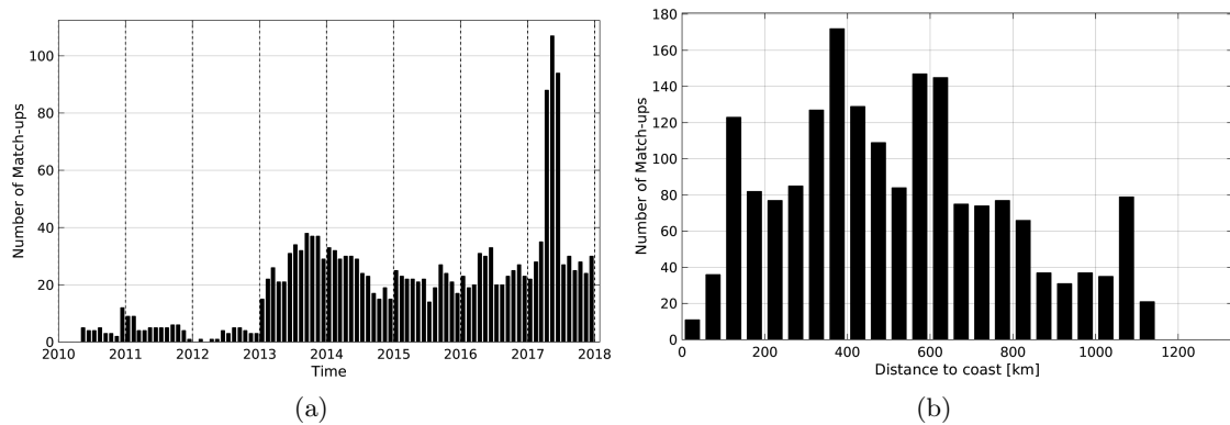
Figure 1: Number of match-ups between Argo and SMOS-L4-CATDS-CECOS-IFREMER-V2-WEEKLY-0.5DEG SSS as a function of time (a) and as function of the distance to coast (b) over the Congo river plume Pi-MEP region and for the full satellite product period.
