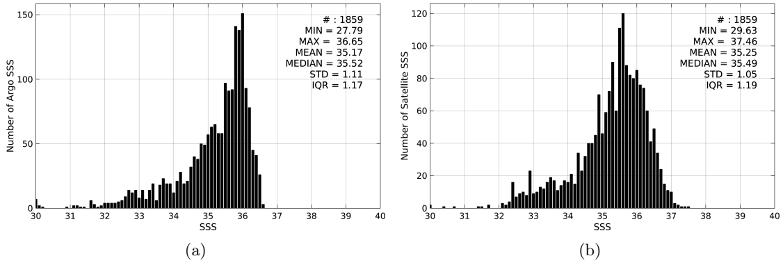
Figure 2: Histograms of SSS from Argo (a) and SMOS-L4-CATDS-CECOS-IFREMER-V2-WEEKLY-0.5DEG (b) considering all match-up pairs per bins of 0.1 over the Congo river plume Pi-MEP region and for the full satellite product period.
