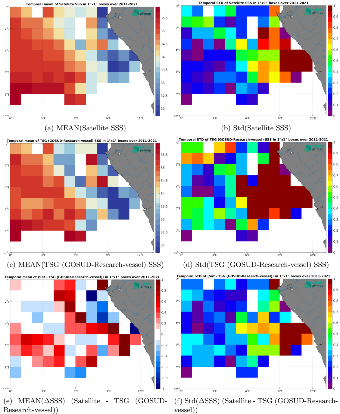
Figure 7: Temporal mean (left) and Std (right) of SSS from SMOS SSS L4 v2 - Daily (BEC) (top), TSG (GOSUD-Research-vessel) (middle), and of \Delta SSS (Satellite - TSG (GOSUD-Research-vessel)). Only match-up pairs are used to generate these maps.
