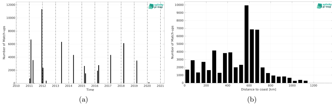
Figure 2: Number of match-ups between TSG (GOSUD-Research-vessel) and SMOS SSS L4 v2 - Daily (BEC) SSS as a function of time (a) and as function of the distance to coast (b) over the Congo river plume Pi-MEP region and for the full satellite product period.
