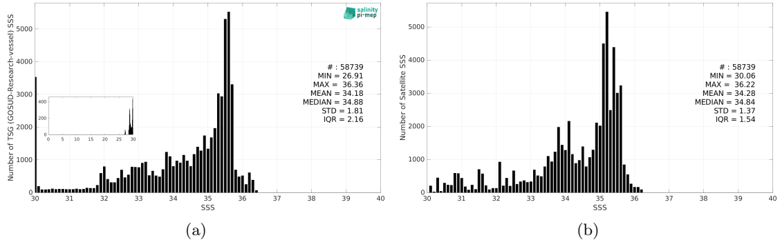
Figure 3: Histograms of SSS from TSG (GOSUD-Research-vessel) (a) and SMOS SSS L4 v2 - Daily (BEC) (b) considering all match-up pairs per bins of 0.1 over the Congo river plume Pi-MEP region and for the full satellite product period.
