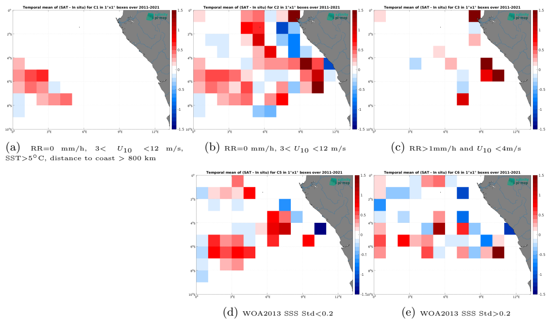
Figure 14: Temporal mean gridded over spatial boxes of size 1^\circ \times 1^\circ of \Delta SSS (SMOS SSS L4 v2 - Daily (BEC) - TSG (GOSUD-Research-vessel)) for 5 different subdatasets corresponding to:RR=0 mm/h, 3 < U_{10} < 12 m/s, SST>5°C, distance to coast > 800 km (a), RR=0 mm/h, 3 < U_{10} < 12 m/s (b), RR>1mm/h and U_{10} < 4 m/s (c), WOA2013 SSS Std<0.2 (d), WOA2013 SSS Std>0.2 (e).
