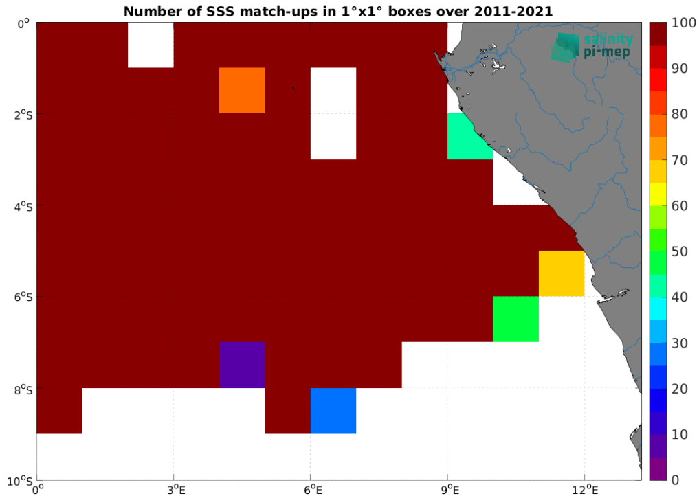
Figure 5: Number of SSS match-ups between TSG (GOSUD-Research-vessel) SSS and the SMOS SSS L4 v2 - Daily (BEC) SSS product for the Congo river plume Pi-MEP region over 1^\circ \times 1^\circ boxes and for the full satellite product period.
