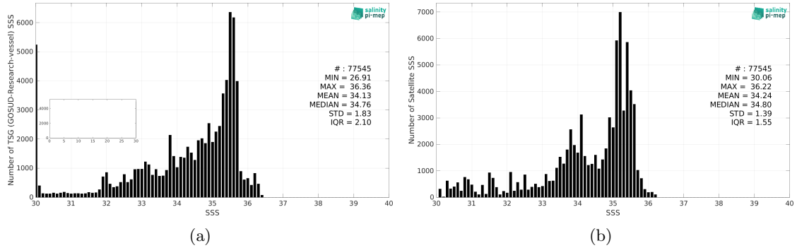
Figure 2: Histograms of SSS from TSG (GOSUD-Research-vessel) (a) and SMOS SSS L4 v2 - Daily (BEC) (b) considering all match-up pairs per bins of 0.1 over the Congo river plume Pi-MEP region and for the full satellite product period.
