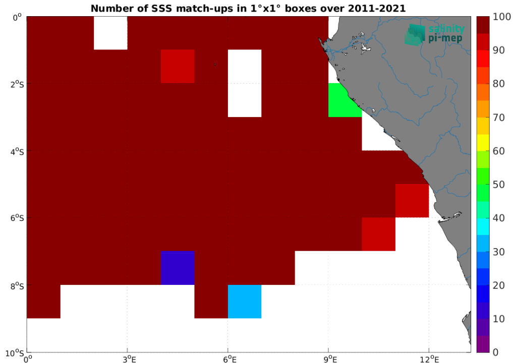
Figure 4: Number of SSS match-ups between TSG (GOSUD-Research-vessel) SSS and the SMOS SSS L4 v2 - Daily (BEC) SSS product for the Congo river plume Pi-MEP region over 1^\circ \times 1^\circ boxes and for the full satellite product period.
