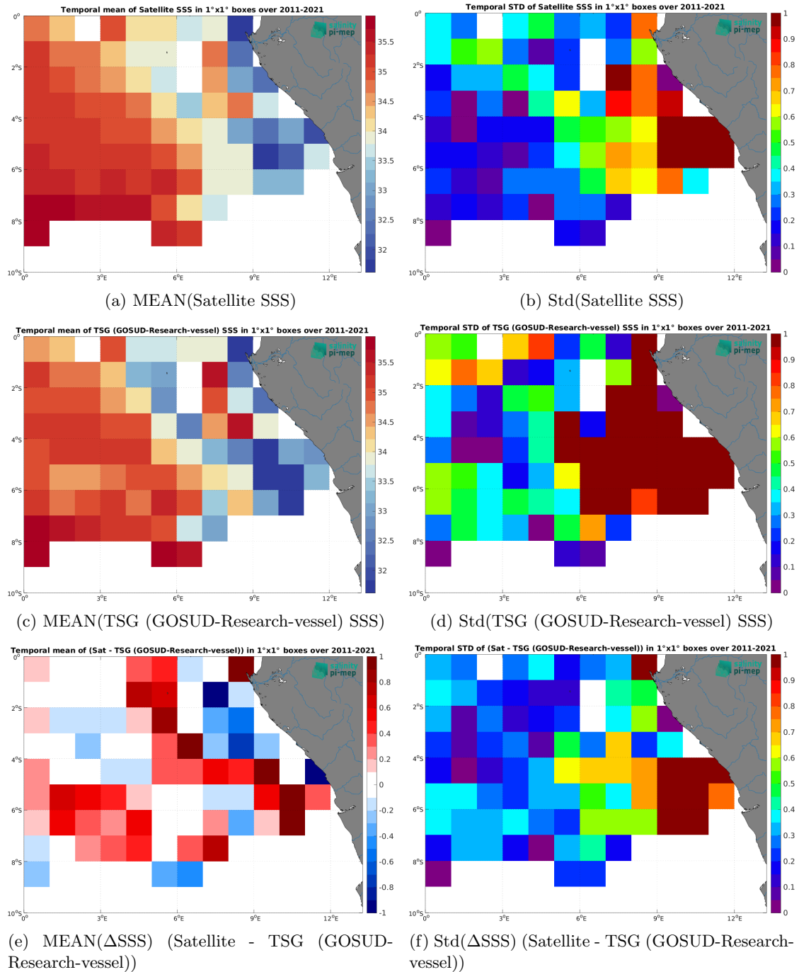
Figure 6: Temporal mean (left) and Std (right) of SSS from SMOS SSS L4 v2 - Daily (BEC) (top), TSG (GOSUD-Research-vessel) (middle), and of \Delta SSS (Satellite - TSG (GOSUD-Research-vessel)). Only match-up pairs are used to generate these maps.
