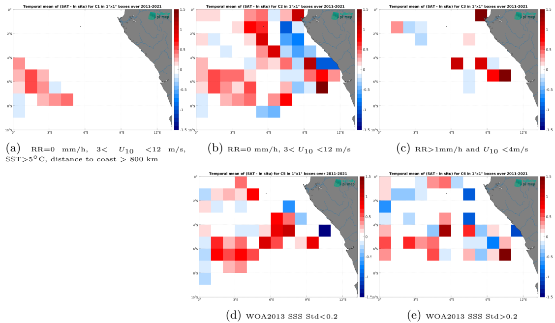
Figure 12: Temporal mean gridded over spatial boxes of size 1^\circ \times 1^\circ of \Delta SSS (SMOS SSS L4 v2 - Daily (BEC) - TSG (GOSUD-Research-vessel)) for 5 different subdatasets corresponding to:RR=0 mm/h, 3 < U_{10} < 12 m/s, SST>5°C, distance to coast > 800 km (a), RR=0 mm/h, 3 < U_{10} < 12 m/s (b), RR>1mm/h and U_{10} < 4 m/s (c), WOA2013 SSS Std<0.2 (d), WOA2013 SSS Std>0.2 (e).
