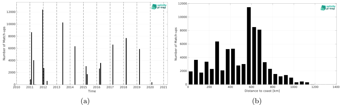
Figure 1: Number of match-ups between TSG (GOSUD-Research-vessel) and SMOS SSS L4 v2 - Daily (BEC) SSS as a function of time (a) and as function of the distance to coast (b) over the Congo river plume Pi-MEP region and for the full satellite product period.
