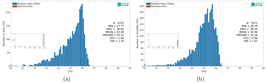
Figure 3: Histograms of SSS from Argo (a) and SMOS SSS L4 v2 - Daily (BEC) (b) considering all match-up pairs per bins of 0.1 over the Congo river plume Pi-MEP region and for the full satellite product period.
