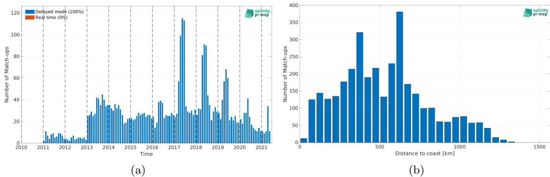
Figure 2: Number of match-ups between Argo and SMOS SSS L4 v2 - Daily (BEC) SSS as a function of time (a) and as function of the distance to coast (b) over the Congo river plume Pi-MEP region and for the full satellite product period.
