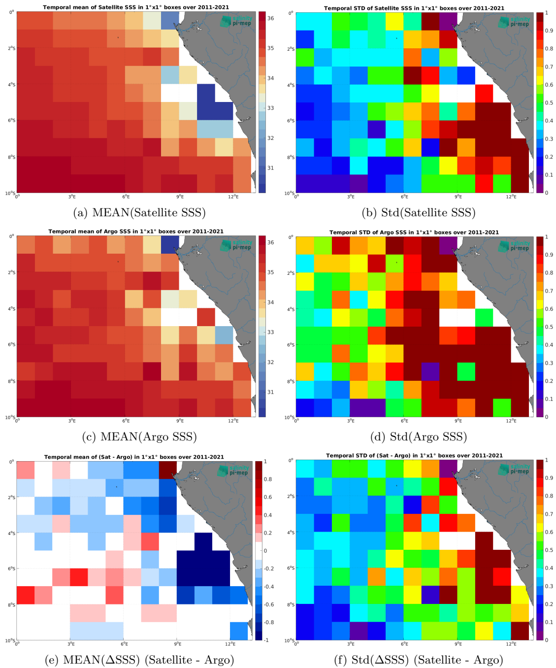
Figure 7: Temporal mean (left) and Std (right) of SSS from SMOS SSS L4 v2 - Daily (BEC) (top), Argo (middle), and of \Delta SSS (Satellite - Argo). Only match-up pairs are used to generate these maps.
