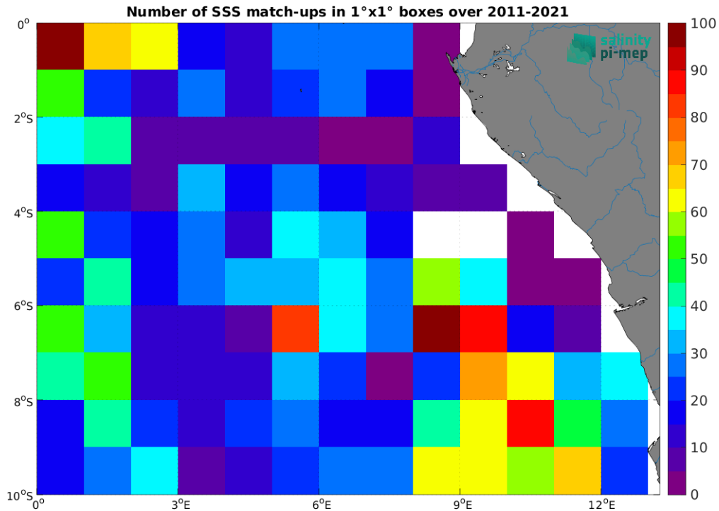
Figure 5: Number of SSS match-ups between Argo SSS and the SMOS SSS L4 v2 - Daily (BEC) SSS product for the Congo river plume Pi-MEP region over 1^\circ \times 1^\circ boxes and for the full satellite product period.
