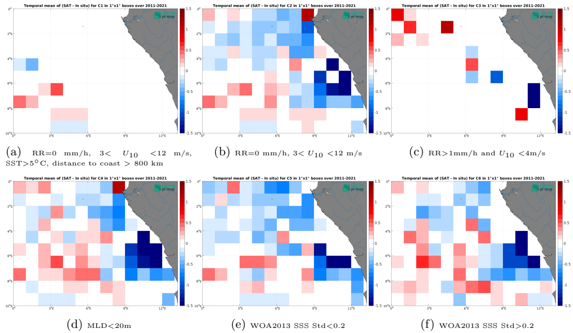
Figure 14: Temporal mean gridded over spatial boxes of size 1^\circ \times 1^\circ of \Delta\text{SSS} (SMOS SSS L4 v2 - Daily (BEC) - Argo) for 6 different subdatasets corresponding to:RR=0 mm/h, 3 < U_{10} < 12 m/s, SST>5°C, distance to coast > 800 km (a), RR=0 mm/h, 3 < U_{10} < 12 m/s (b), RR>1mm/h and U_{10} < 4 m/s (c),MLD<20m (d),WOA2013 SSS Std<0.2 (e),WOA2013 SSS Std>0.2 (f).
