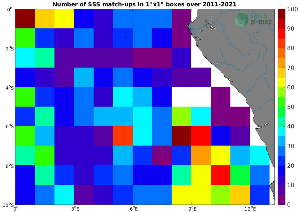
Figure 4: Number of SSS match-ups between Argo SSS and the SMOS SSS L4 v2 - Daily (BEC) SSS product for the Congo river plume Pi-MEP region over 1^\circ \times 1^\circ boxes and for the full satellite product period.
