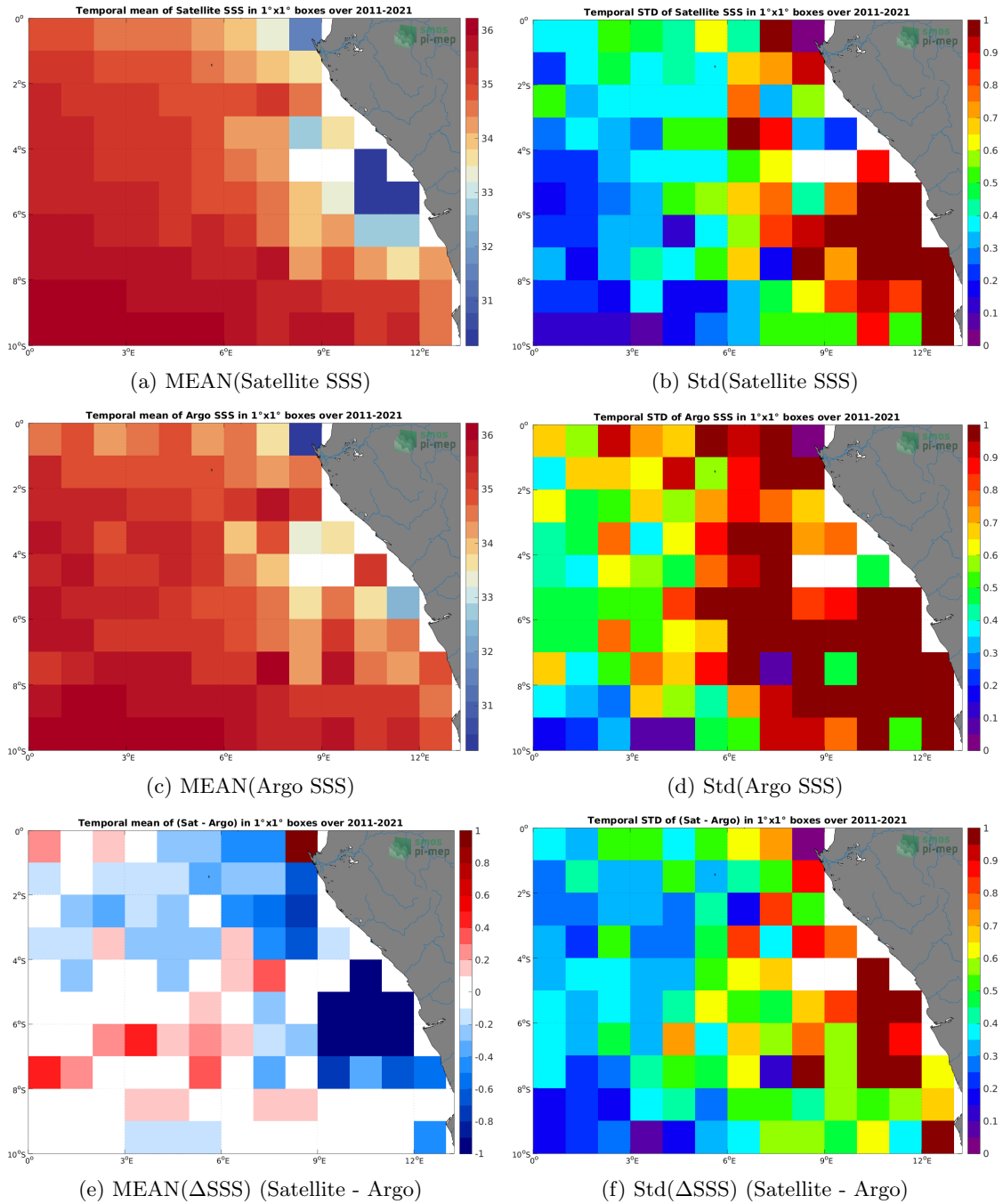
Figure 6: Temporal mean (left) and Std (right) of SSS from SMOS SSS L4 v2 - Daily (BEC) (top), Argo (middle), and of \Delta SSS (Satellite - Argo). Only match-up pairs are used to generate these maps.
