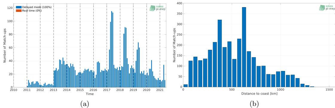
Figure 1: Number of match-ups between Argo and SMOS SSS L4 v2 - Daily (BEC) SSS as a function of time (a) and as function of the distance to coast (b) over the Congo river plume Pi-MEP region and for the full satellite product period.
