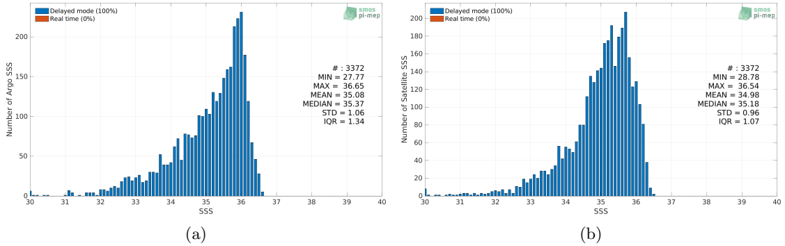
Figure 2: Histograms of SSS from Argo (a) and SMOS SSS L4 v2 - Daily (BEC) (b) considering all match-up pairs per bins of 0.1 over the Congo river plume Pi-MEP region and for the full satellite product period.
