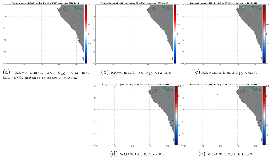
Figure 12: Temporal mean gridded over spatial boxes of size 1^{\circ}\times 1^{\circ} of \Delta\text{SSS} (SMOS-L3-ICDC-V3-MONTHLY-0.5DEG - TSG-POLARSTERN) for 5 different subdatasets corresponding to:RR=0 mm/h, 3 < U_{10} < 12 m/s, SST > 5^{\circ}\text{C} , distance to coast > 800 km (a), RR=0 mm/h, 3 < U_{10} < 12 m/s (b), RR > 1 mm/h and U_{10} < 4 m/s (c), WOA2013 SSS Std < 0.2 (d), WOA2013 SSS Std > 0.2 (e).
