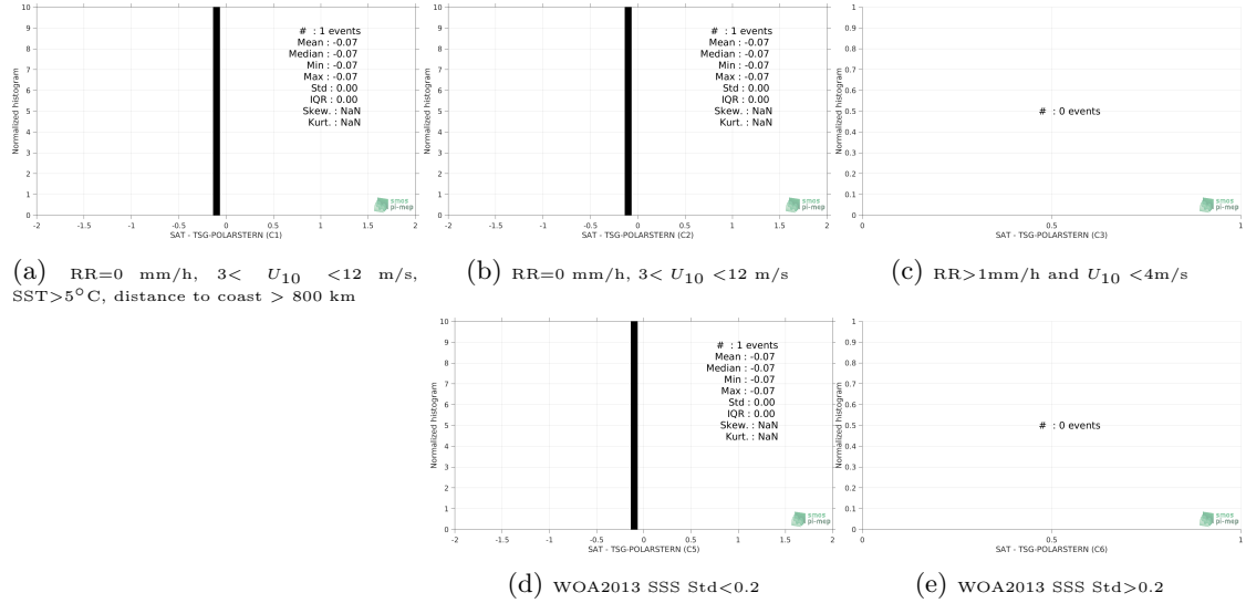
Figure 13: Normalized histogram of \Delta\text{SSS} (SMOS-L3-ICDC-V3-MONTHLY-0.5DEG - TSG-POLARSTERN) for 5 different subdatasets corresponding to: RR=0 mm/h, 3 < U_{10} < 12 m/s, SST > 5^\circ\text{C} , distance to coast > 800 km (a), RR=0 mm/h, 3 < U_{10} < 12 m/s (b), RR > 1\text{mm/h} and U_{10} < 4\text{m/s} (c), WOA2013 SSS Std < 0.2 (d), WOA2013 SSS Std > 0.2 (e).
