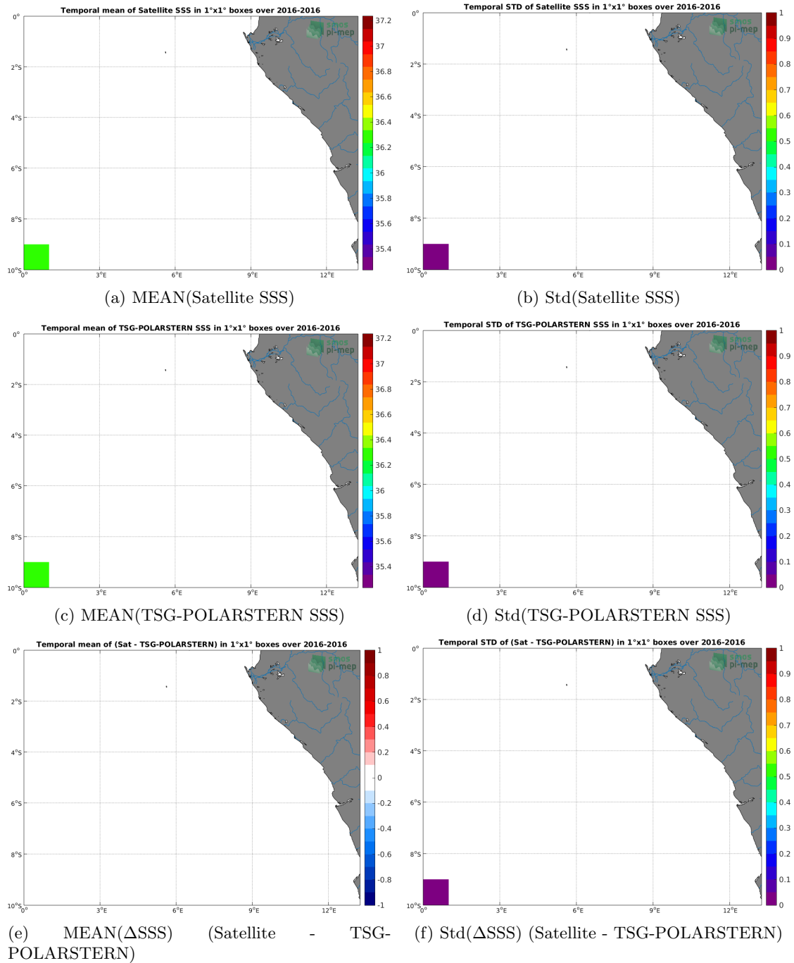
Figure 6: Temporal mean (left) and Std (right) of SSS from SMOS-L3-ICDC-V3-MONTHLY-0.5DEG (top), TSG-POLARSTERN (middle), and of \Delta SSS (Satellite - TSG-POLARSTERN). Only match-up pairs are used to generate these maps.
