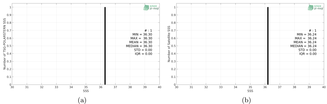
Figure 2: Histograms of SSS from TSG-POLARSTERN (a) and SMOS-L3-ICDC-V3-MONTHLY-0.5DEG (b) considering all match-up pairs per bins of 0.1 over the Congo river plume Pi-MEP region and for the full satellite product period.
