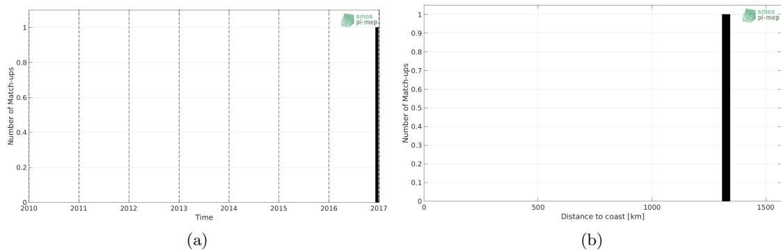
Figure 1: Number of match-ups between TSG-POLARSTERN and SMOS-L3-ICDC-V3-MONTHLY-0.5DEG SSS as a function of time (a) and as function of the distance to coast (b) over the Congo river plume Pi-MEP region and for the full satellite product period.
