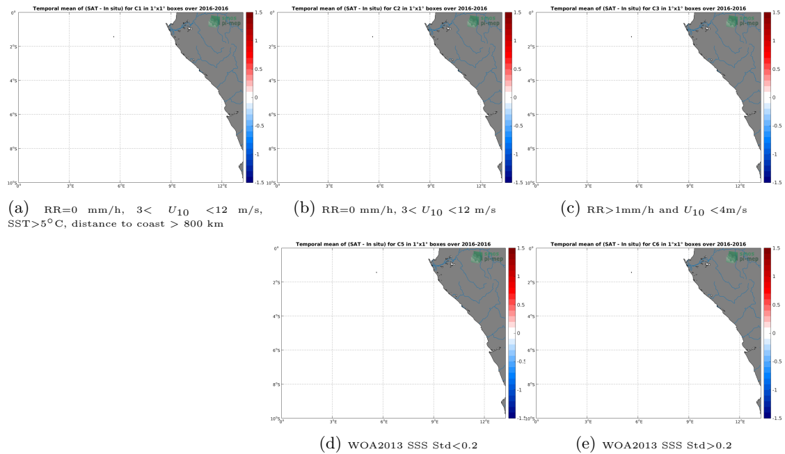
Figure 12: Temporal mean gridded over spatial boxes of size 1^\circ \times 1^\circ of \Delta SSS (SMOS-L3-ICDC-V3-MONTHLY-0.5DEG - TSG-POLARSTERN) for 5 different subdatasets corresponding to:RR=0 mm/h, 3 < U_{10} < 12 m/s, SST > 5^\circ\text{C} , distance to coast > 800 km (a), RR=0 mm/h, 3 < U_{10} < 12 m/s (b), RR > 1 mm/h and U_{10} < 4 m/s (c), WOA2013 SSS Std < 0.2 (d), WOA2013 SSS Std > 0.2 (e).
