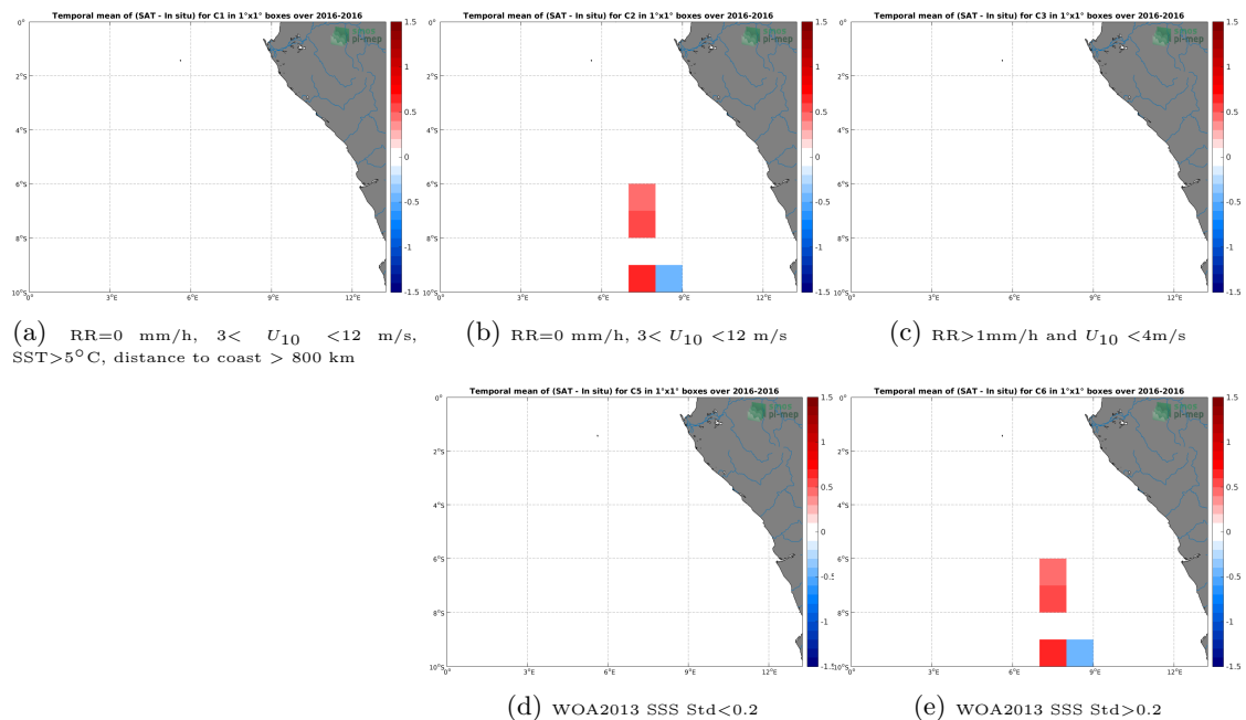
Figure 12: Temporal mean gridded over spatial boxes of size 1^\circ \times 1^\circ of \Delta\text{SSS} (SMOS SSS L3 v3 Monthly (ICDC) - TSG (LEGOS-DM)) for 5 different subdatasets corresponding to:RR=0 mm/h, 3 < U_{10} < 12 m/s, SST >5^\circ\text{C} , distance to coast > 800 km (a), RR=0 mm/h, 3 < U_{10} < 12 m/s (b), RR >1 mm/h and U_{10} < 4 m/s (c), WOA2013 SSS Std <0.2 (d), WOA2013 SSS Std >0.2 (e).
