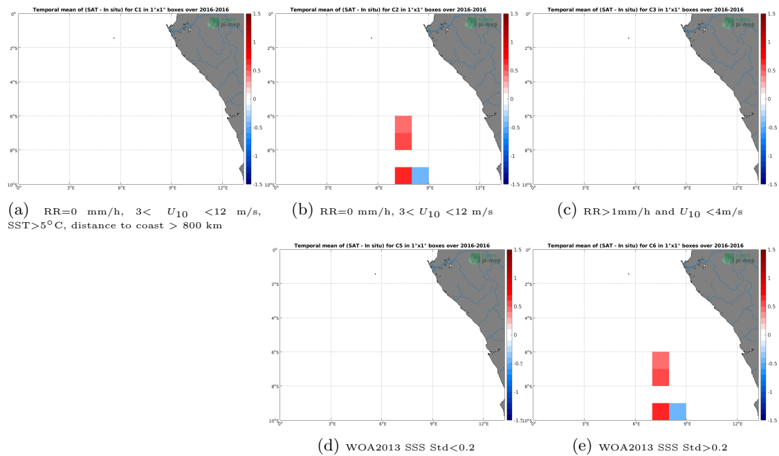
Figure 12: Temporal mean gridded over spatial boxes of size 1^\circ \times 1^\circ of \Delta SSS (SMOS SSS L3 v3 Monthly (ICDC) - TSG (LEGOS-DM)) for 5 different subdatasets corresponding to:RR=0 mm/h, 3 < U_{10} < 12 m/s, SST >5^\circ\text{C} , distance to coast > 800 km (a), RR=0 mm/h, 3 < U_{10} < 12 m/s (b), RR >1 mm/h and U_{10} < 4 m/s (c), WOA2013 SSS Std <0.2 (d), WOA2013 SSS Std >0.2 (e).
