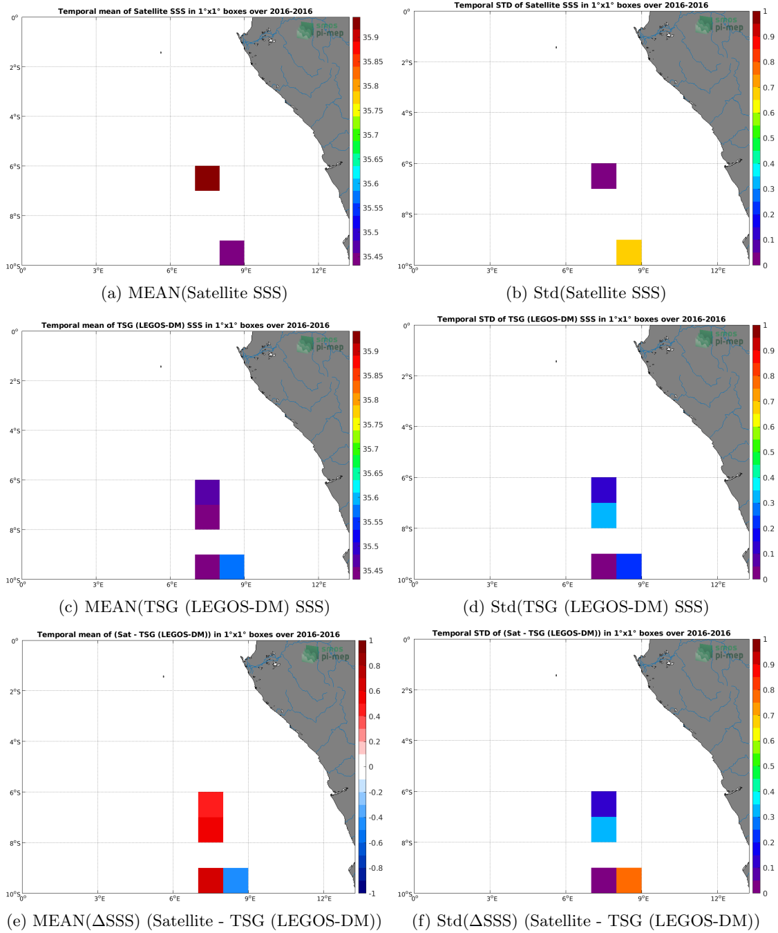
Figure 6: Temporal mean (left) and Std (right) of SSS from SMOS SSS L3 v3 Monthly (ICDC) (top), TSG (LEGOS-DM) (middle), and of \Delta SSS (Satellite - TSG (LEGOS-DM)). Only match-up pairs are used to generate these maps.
