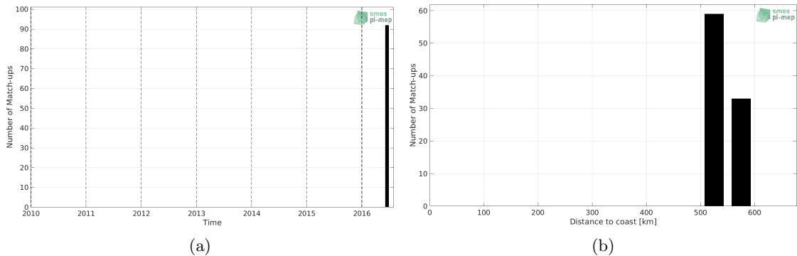
Figure 1: Number of match-ups between TSG (LEGOS-DM) and SMOS SSS L3 v3 Monthly (ICDC) SSS as a function of time (a) and as function of the distance to coast (b) over the Congo river plume Pi-MEP region and for the full satellite product period.
