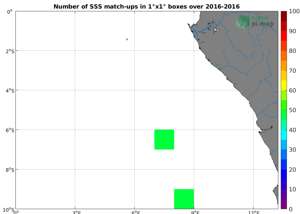
Figure 4: Number of SSS match-ups between TSG (LEGOS-DM) SSS and the SMOS SSS L3 v3 Monthly (ICDC) SSS product for the Congo river plume Pi-MEP region over 1°x1° boxes and for the full satellite product period.
