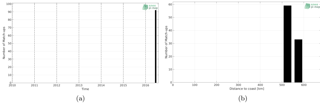
Figure 1: Number of match-ups between TSG-LEGOS-DM and SMOS-L3-ICDC-V3-MONTHLY-0.5DEG SSS as a function of time (a) and as function of the distance to coast (b) over the Congo river plume Pi-MEP region and for the full satellite product period.
