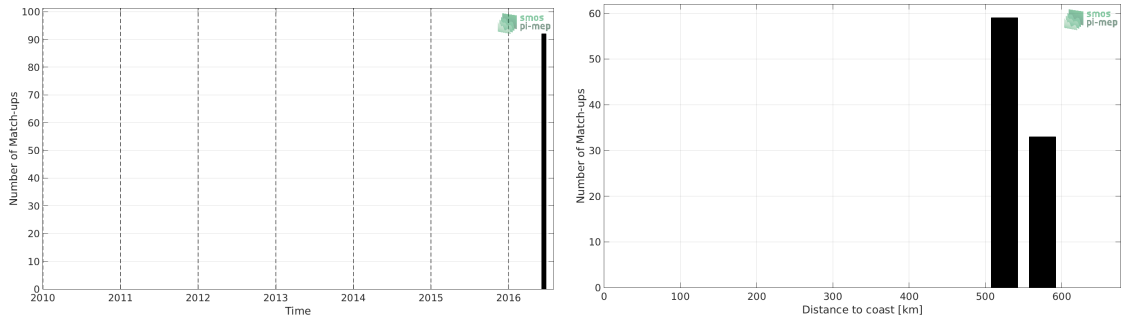
Figure 1: Number of match-ups between TSG-LEGOS-DM and SMOS-L3-ICDC-V3-MONTHLY-0.5DEG SSS as a function of time (a) and as function of the distance to coast (b) over the Congo river plume Pi-MEP region and for the full satellite product period.
