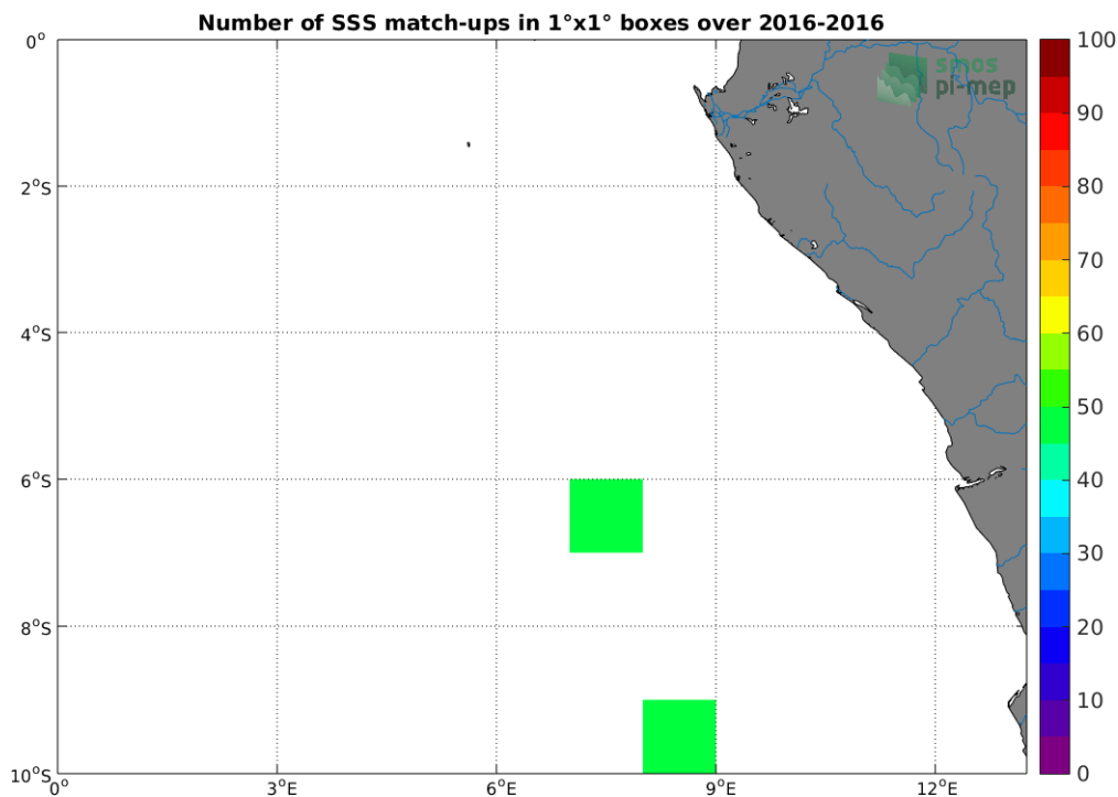
Figure 4: Number of SSS match-ups between TSG-LEGOS-DM SSS and the SMOS-L3-ICDC-V3-MONTHLY-0.5DEG SSS product for the Congo river plume Pi-MEP region over 1°x1° boxes and for the full satellite product period.
