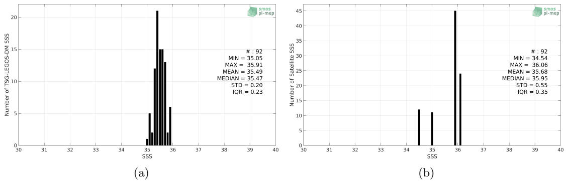
Figure 2: Histograms of SSS from TSG-LEGOS-DM (a) and SMOS-L3-ICDC-V3-MONTHLY-0.5DEG (b) considering all match-up pairs per bins of 0.1 over the Congo river plume Pi-MEP region and for the full satellite product period.
