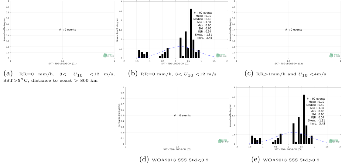
Figure 13: Normalized histogram of \Delta SSS (SMOS-L3-ICDC-V3-MONTHLY-0.5DEG - TSG-LEGOS-DM) for 5 different subdatasets corresponding to: RR=0 mm/h, 3 < U_{10} < 12 m/s, SST >5^{\circ} C, distance to coast > 800 km (a), RR=0 mm/h, 3 < U_{10} < 12 m/s (b), RR >1 mm/h and U_{10} < 4 m/s (c), WOA2013 SSS Std <0.2 (d), WOA2013 SSS Std >0.2 (e).
