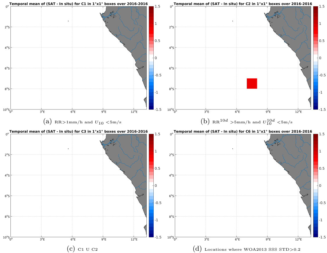
Figure 12: Temporal mean gridded over spatial boxes of size 1^\circ \times 1^\circ of \Delta SSS (SMOS-L3-ICDC-V3-MONTHLY-0.5DEG - TSG-LEGOS-DM) for 4 different subdatasets corresponding to: RR > 1\text{mm/h} and U_{10} < 5\text{m/s} (a), RR^{10d} > 5\text{mm/h} and U_{10}^{10d} < 5\text{m/s} (b), C1 \cup C2 (c), Locations where WOA2013 SSS STD > 0.2 (d).
