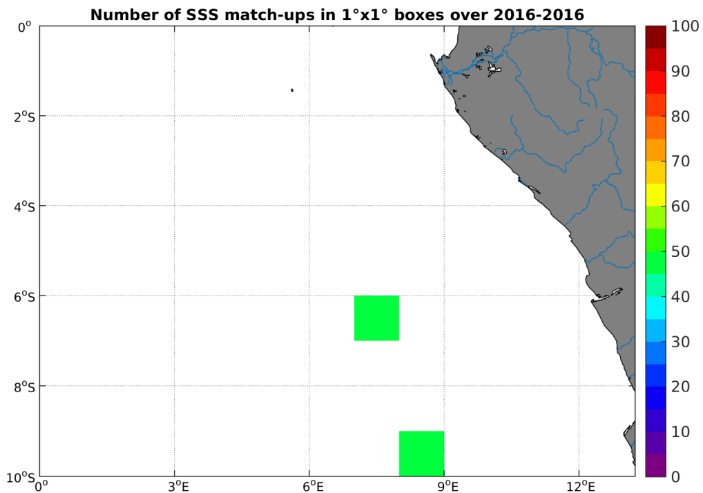
Figure 4: Number of SSS match-ups between TSG-LEGOS-DM SSS and the SMOS-L3-ICDC-V3-MONTHLY-0.5DEG SSS product for the Congo river plume Pi-MEP region over 1^\circ \times 1^\circ boxes and for the full satellite product period.
