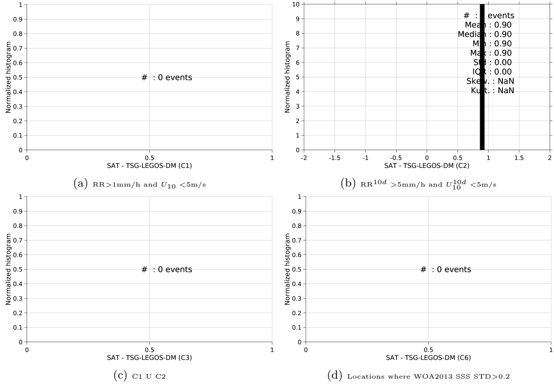
Figure 13: Normalized histogram of \Delta\text{SSS} (SMOS-L3-ICDC-V3-MONTHLY-0.5DEG - TSG-LEGOS-DM) for 6 different subdatasets corresponding to: RR > 1\text{mm/h} and U_{10} < 5\text{m/s} (a), RR^{10d} > 5\text{mm/h} and U_{10}^{10d} < 5\text{m/s} (b), C1 U C2 (c), Locations where WOA2013 SSS STD > 0.2 (d).
