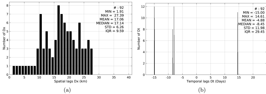
Figure 5: Histograms of the spatial (a) and temporal (b) lags between the time of the TSG-LEGOS-DM measurements and the date of the corresponding SMOS-L3-ICDC-V3-MONTHLY-0.5DEG SSS product.
