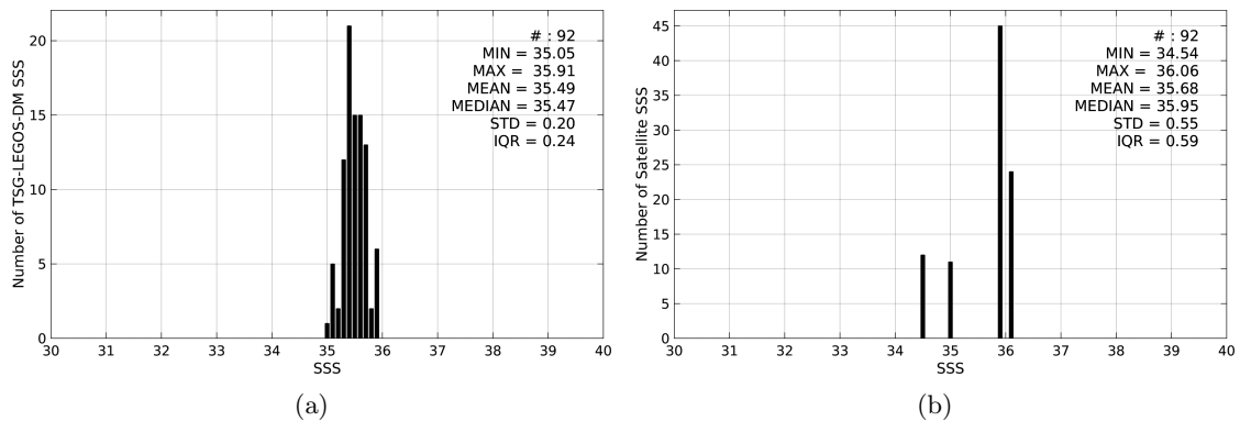
Figure 2: Histograms of SSS from TSG-LEGOS-DM (a) and SMOS-L3-ICDC-V3-MONTHLY-0.5DEG (b) considering all match-up pairs per bins of 0.1 over the Congo river plume Pi-MEP region and for the full satellite product period.
