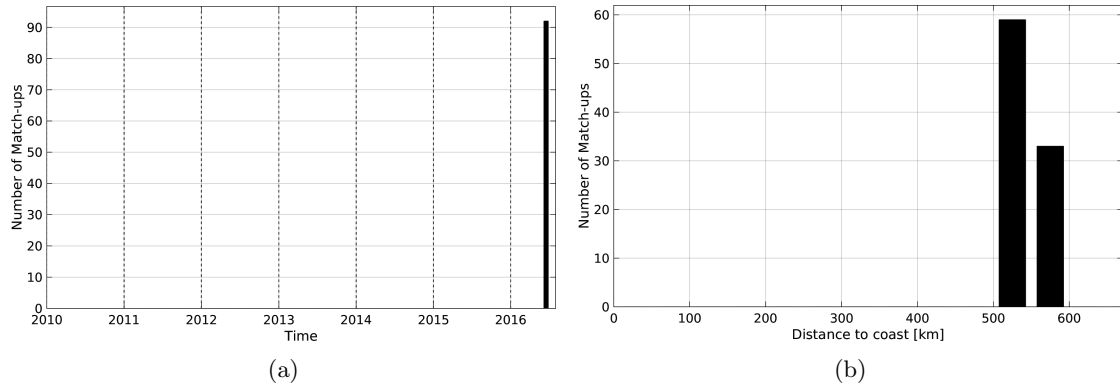
Figure 1: Number of match-ups between TSG-LEGOS-DM and SMOS-L3-ICDC-V3-MONTHLY-0.5DEG SSS as a function of time (a) and as function of the distance to coast (b) over the Congo river plume Pi-MEP region and for the full satellite product period.
