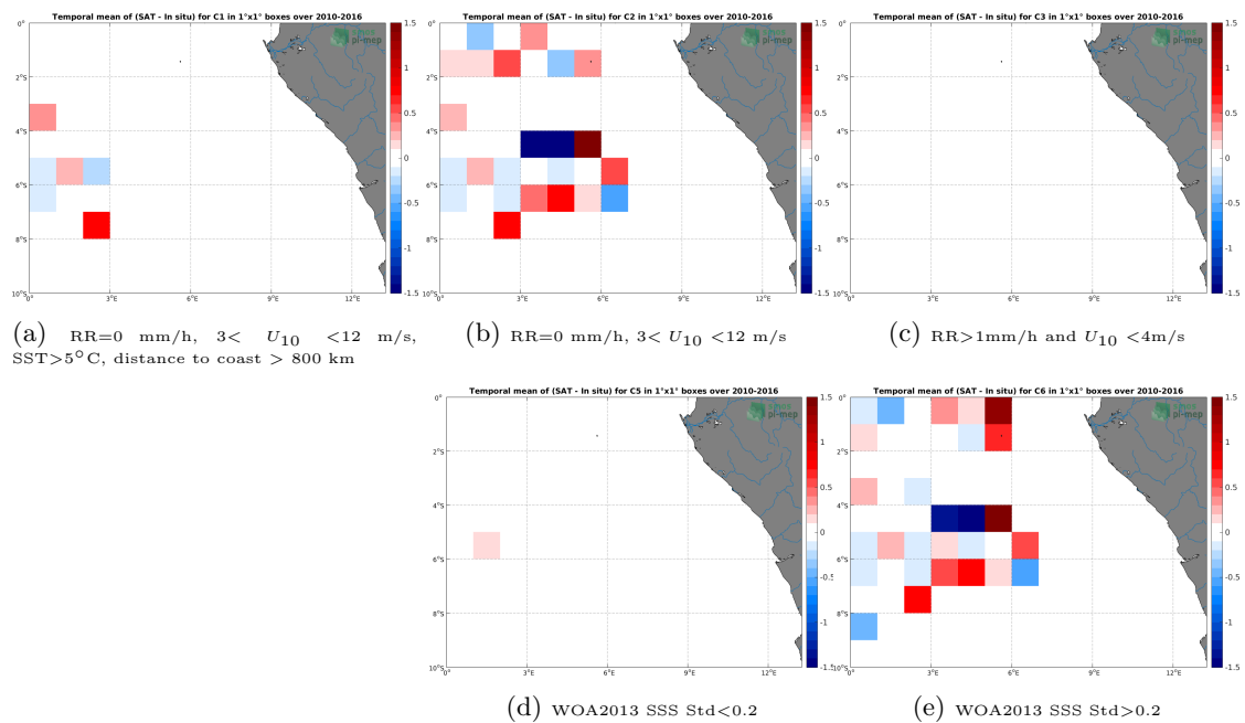
Figure 12: Temporal mean gridded over spatial boxes of size 1^\circ \times 1^\circ of \Delta\text{SSS} (SMOS SSS L3 v3 Monthly (ICDC) - TSG (GOSUD-Research-vessel)) for 5 different subdatasets corresponding to:RR=0 mm/h, 3 < U_{10} < 12 m/s, SST>5°C, distance to coast > 800 km (a), RR=0 mm/h, 3 < U_{10} < 12 m/s (b), RR>1mm/h and U_{10} < 4 m/s (c), WOA2013 SSS Std<0.2 (d), WOA2013 SSS Std>0.2 (e).
