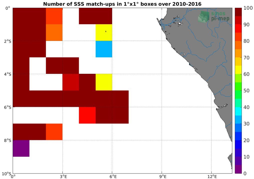
Figure 4: Number of SSS match-ups between TSG (GOSUD-Research-vessel) SSS and the SMOS SSS L3 v3 Monthly (ICDC) SSS product for the Congo river plume Pi-MEP region over 1^{\circ} \times 1^{\circ} boxes and for the full satellite product period.
