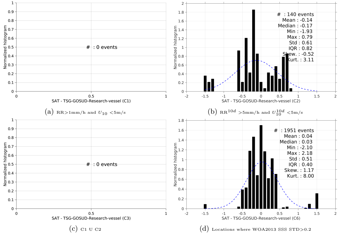
Figure 13: Normalized histogram of \Delta\text{SSS} (SMOS-L3-ICDC-V3-MONTHLY-0.5DEG - TSG-GOSUD-Research-vessel) for 6 different subdatasets corresponding to: RR > 1\text{mm/h} and U_{10} < 5\text{m/s} (a), RR^{10d} > 5\text{mm/h} and U_{10}^{10d} < 5\text{m/s} (b), C1 \cup C2 (c), Locations where WOA2013 SSS STD > 0.2 (d).
