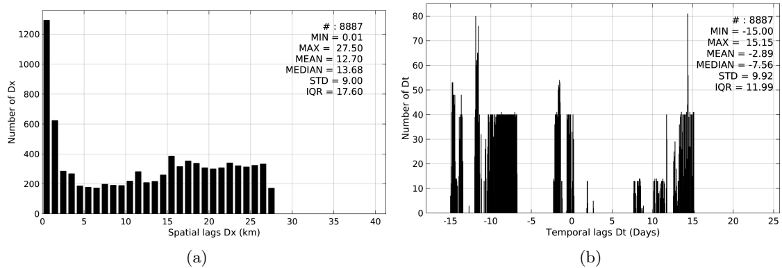
Figure 5: Histograms of the spatial (a) and temporal (b) lags between the time of the TSG-GOSUD-Research-vessel measurements and the date of the corresponding SMOS-L3-ICDC-V3-MONTHLY-0.5DEG SSS product.
