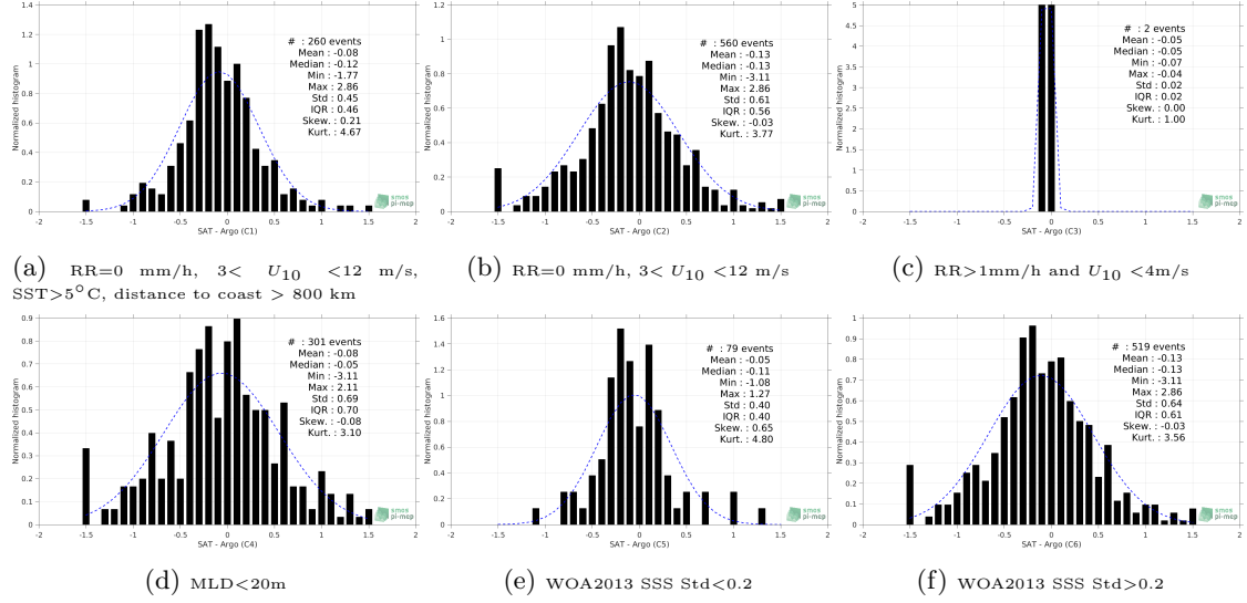
Figure 13: Normalized histogram of \Delta SSS (SMOS SSS L3 v3 Monthly (ICDC) - Argo) for 6 different subdatasets corresponding to: RR=0 mm/h, 3 < U_{10} < 12 m/s, SST>5°C, distance to coast > 800 km (a), RR=0 mm/h, 3 < U_{10} < 12 m/s (b), RR>1mm/h and U_{10} < 4 m/s (c), MLD<20m (d), WOA2013 SSS Std<0.2 (e), WOA2013 SSS Std>0.2 (f).
