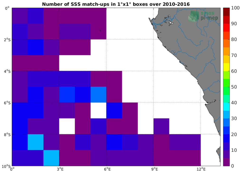
Figure 4: Number of SSS match-ups between Argo SSS and the SMOS-L3-ICDC-V3-MONTHLY-0.5DEG SSS product for the Congo river plume Pi-MEP region over 1°x1° boxes and for the full satellite product period.
