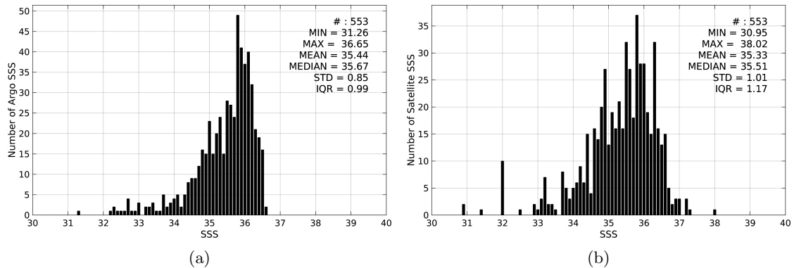
Figure 2: Histograms of SSS from Argo (a) and SMOS-L3-ICDC-V3-MONTHLY-0.5DEG (b) considering all match-up pairs per bins of 0.1 over the Congo river plume Pi-MEP region and for the full satellite product period.
