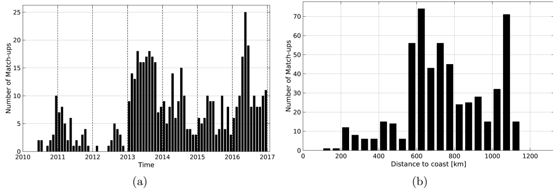
Figure 1: Number of match-ups between Argo and SMOS-L3-ICDC-V3-MONTHLY-0.5DEG SSS as a function of time (a) and as function of the distance to coast (b) over the Congo river plume Pi-MEP region and for the full satellite product period.
