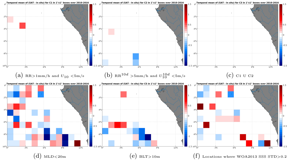
Figure 12: Temporal mean gridded over spatial boxes of size 1^\circ \times 1^\circ of \Delta SSS (SMOS-L3-ICDC-V3-MONTHLY-0.5DEG - Argo) for 6 different subdatasets corresponding to:RR >1 mm/h and U_{10} < 5 m/s (a), RR^{10d} > 5 mm/h and U_{10}^{10d} < 5 m/s (b), C1 U C2 (c),MLD <20 m (d),BLT >10 m (e),Locations where WOA2013 SSS STD >0.2 (f).
