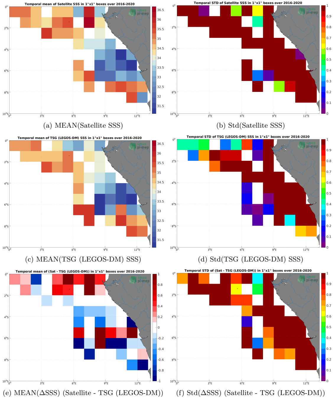
Figure 6: Temporal mean (left) and Std (right) of SSS from SMOS SSS L2Q v331 - With FLAG (CMEMS-CATDS-CPDC) (top), TSG (LEGOS-DM) (middle), and of \Delta SSS (Satellite - TSG (LEGOS-DM)). Only match-up pairs are used to generate these maps.
