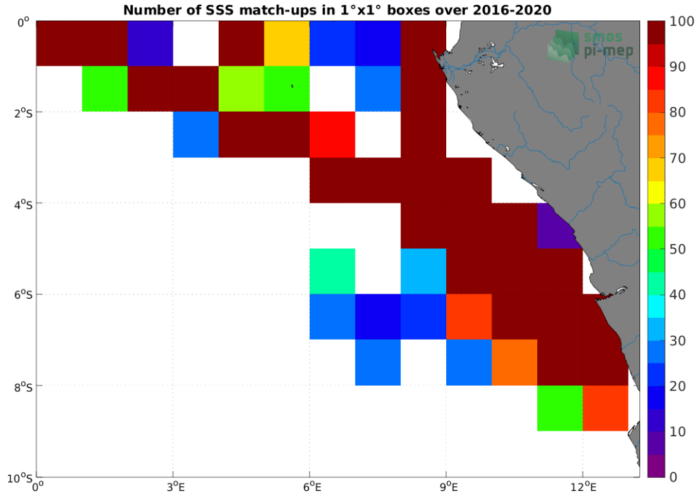
Figure 4: Number of SSS match-ups between TSG (LEGOS-DM) SSS and the SMOS SSS L2Q v331 - With FLAG (CMEMS-CATDS-CPDC) SSS product for the Congo river plume Pi-MEP region over 1^\circ \times 1^\circ boxes and for the full satellite product period.
