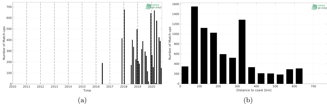
Figure 1: Number of match-ups between TSG (LEGOS-DM) and SMOS SSS L2Q v331 - With FLAG (CMEMS-CATDS-CPDC) SSS as a function of time (a) and as function of the distance to coast (b) over the Congo river plume Pi-MEP region and for the full satellite product period.
