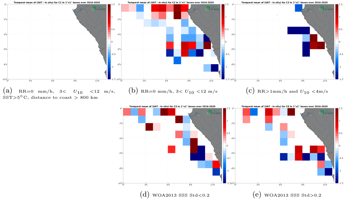
Figure 12: Temporal mean gridded over spatial boxes of size 1^{\circ}\times 1^{\circ} of \Delta\text{SSS} (SMOS SSS L2Q v331 - With FLAG (CMEMS-CATDS-CPDC) - TSG (LEGOS-DM)) for 5 different subdatasets corresponding to:RR=0 mm/h, 3 < U_{10} < 12 m/s, SST >5^{\circ}\text{C} , distance to coast > 800 km (a), RR=0 mm/h, 3 < U_{10} < 12 m/s (b), RR >1 mm/h and U_{10} < 4 m/s (c), WOA2013 SSS Std <0.2 (d), WOA2013 SSS Std >0.2 (e).
