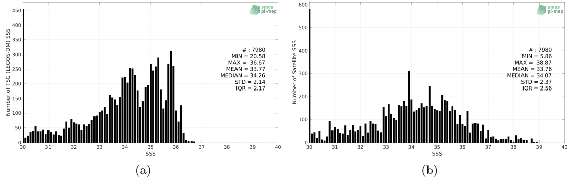
Figure 2: Histograms of SSS from TSG (LEGOS-DM) (a) and SMOS SSS L2Q v331 - With FLAG (CMEMS-CATDS-CPDC) (b) considering all match-up pairs per bins of 0.1 over the Congo river plume Pi-MEP region and for the full satellite product period.
