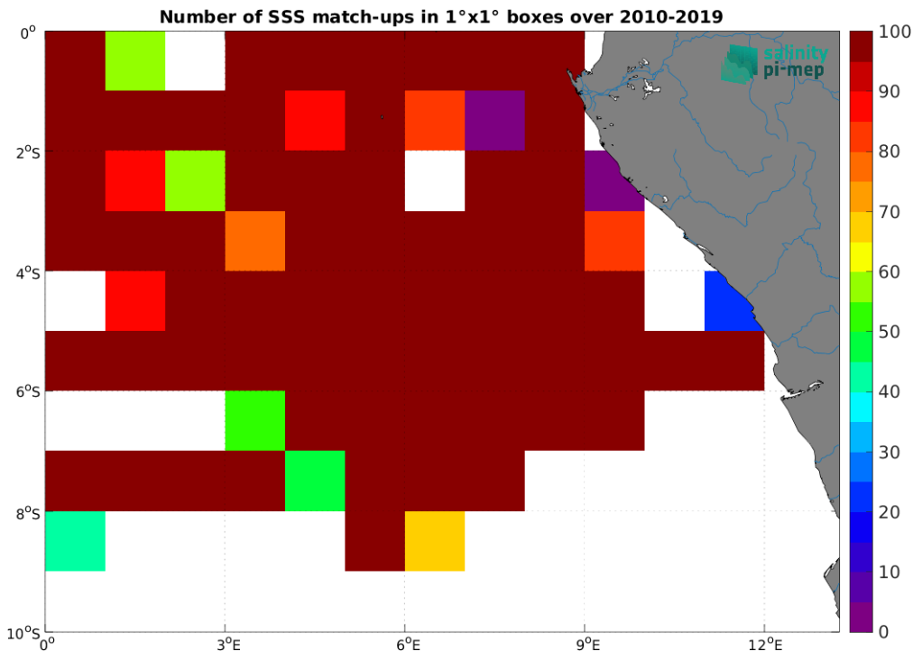
Figure 5: Number of SSS match-ups between TSG (GOSUD-Research-vessel) SSS and the SMOS SSS L2Q v331 - With FLAG (CMEMS-CATDS-CPDC) SSS product for the Congo river plume Pi-MEP region over 1^\circ \times 1^\circ boxes and for the full satellite product period.
