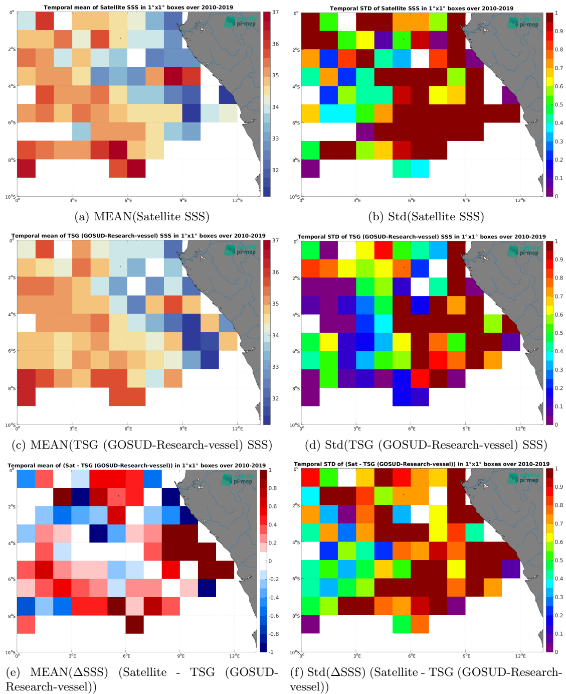
Figure 7: Temporal mean (left) and Std (right) of SSS from SMOS SSS L2Q v331 - With FLAG (CMEMS-CATDS-CPDC) (top), TSG (GOSUD-Research-vessel) (middle), and of \Delta SSS (Satellite - TSG (GOSUD-Research-vessel)). Only match-up pairs are used to generate these maps.
