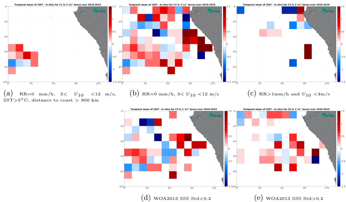
Figure 14: Temporal mean gridded over spatial boxes of size 1^\circ \times 1^\circ of \Delta SSS (SMOS SSS L2Q v331 - With FLAG (CMEMS-CATDS-CPDC) - TSG (GOSUD-Research-vessel)) for 5 different subdatasets corresponding to:RR=0 mm/h, 3 < U_{10} < 12 m/s, SST > 5^\circ\text{C} , distance to coast > 800 km (a), RR=0 mm/h, 3 < U_{10} < 12 m/s (b), RR > 1 mm/h and U_{10} < 4 m/s (c), WOA2013 SSS Std < 0.2 (d), WOA2013 SSS Std > 0.2 (e).
