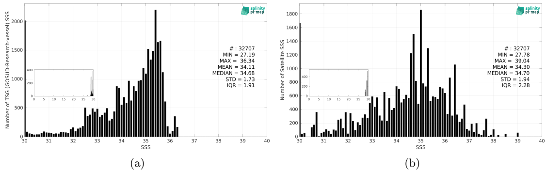
Figure 3: Histograms of SSS from TSG (GOSUD-Research-vessel) (a) and SMOS SSS L2Q v331 - With FLAG (CMEMS-CATDS-CPDC) (b) considering all match-up pairs per bins of 0.1 over the Congo river plume Pi-MEP region and for the full satellite product period.
