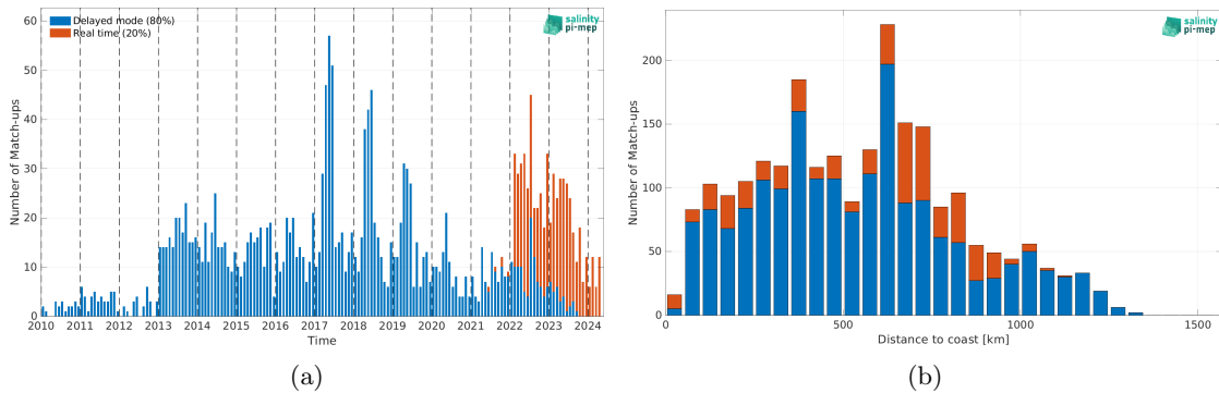
Figure 2: Number of match-ups between Argo and SMOS SSS L2Q v331 - With FLAG (CMEMS-CATDS-CPDC) SSS as a function of time (a) and as function of the distance to coast (b) over the Congo river plume Pi-MEP region and for the full satellite product period.
