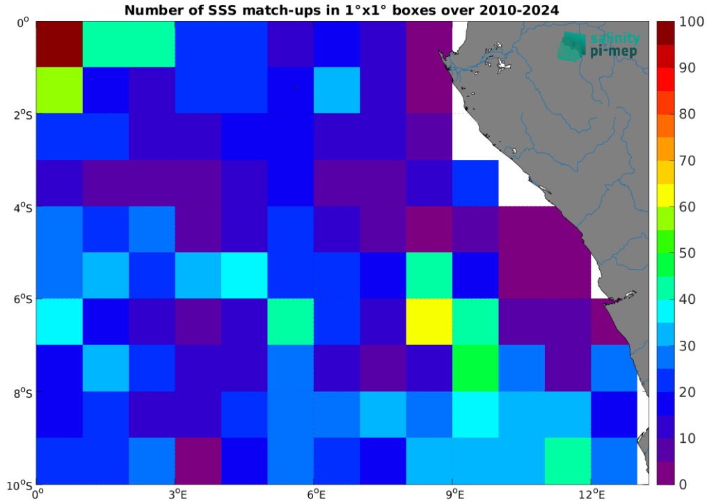
Figure 5: Number of SSS match-ups between Argo SSS and the SMOS SSS L2Q v331 - With FLAG (CMEMS-CATDS-CPDC) SSS product for the Congo river plume Pi-MEP region over 1^\circ \times 1^\circ boxes and for the full satellite product period.
