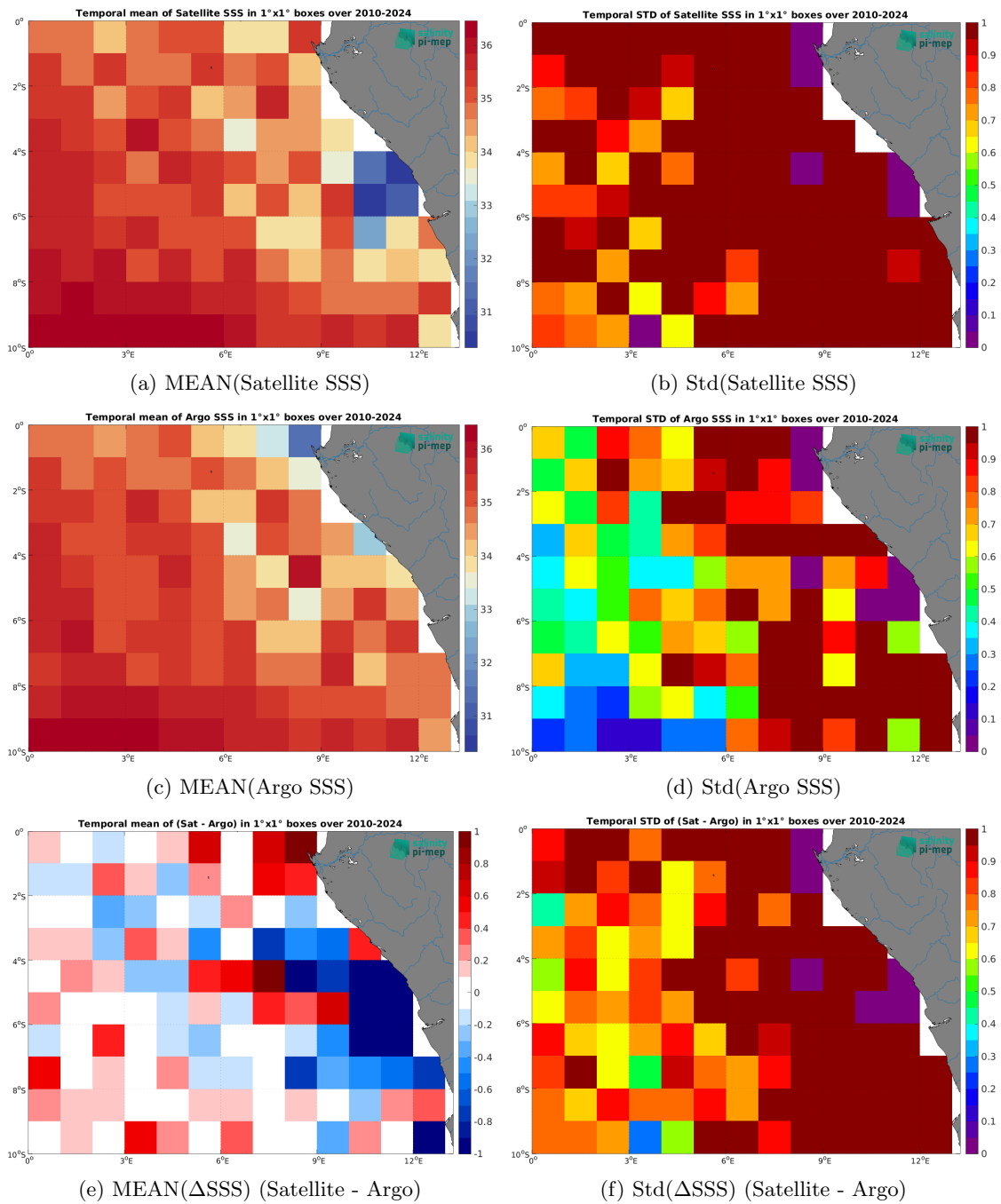
Figure 7: Temporal mean (left) and Std (right) of SSS from SMOS SSS L2Q v331 - With FLAG (CMEMS-CATDS-CPDC) (top), Argo (middle), and of \Delta SSS (Satellite - Argo). Only match-up pairs are used to generate these maps.
