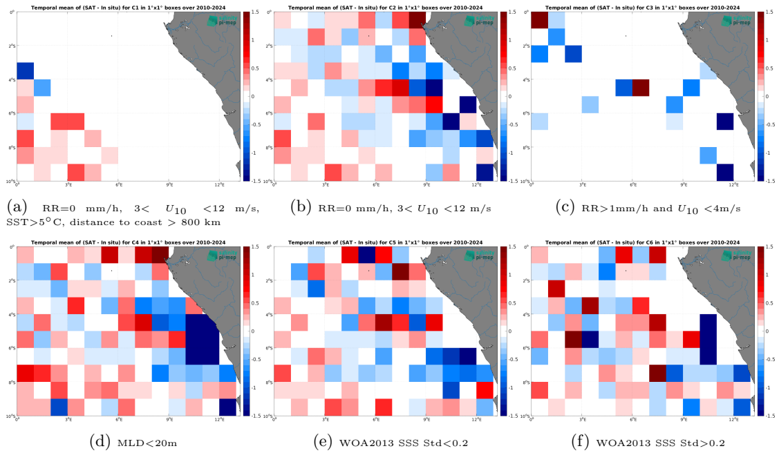
Figure 14: Temporal mean gridded over spatial boxes of size 1^\circ \times 1^\circ of \Delta SSS (SMOS SSS L2Q v331 - With FLAG (CMEMS-CATDS-CPDC) - Argo) for 6 different subdatasets corresponding to:RR=0 mm/h, 3 < U_{10} < 12 m/s, SST>5°C, distance to coast > 800 km (a), RR=0 mm/h, 3 < U_{10} < 12 m/s (b), RR>1mm/h and U_{10} < 4 m/s (c),MLD<20m (d),WOA2013 SSS Std<0.2 (e),WOA2013 SSS Std>0.2 (f).
