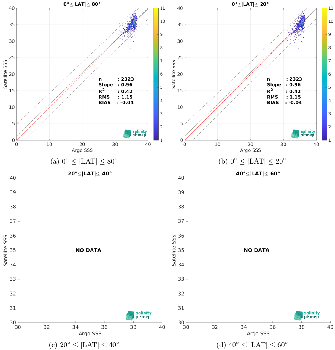
Figure 10: Contour maps of the concentration of SMOS SSS L2Q v331 - With FLAG (CMEMS-CATDS-CPDC) SSS ( y -axis) versus Argo SSS ( x -axis) at match-up pairs for different latitude bands. For each plot, the red line shows x=y . The black thin and dashed lines indicate a linear fit through the data cloud and the \pm 95\% confidence levels, respectively. The number match-up pairs n , the slope and R^2 coefficient of the linear fit, the root mean square (RMS) and the mean bias between satellite and in situ data are indicated for each latitude band in each plots.
