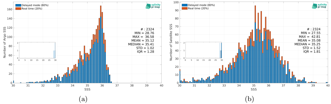
Figure 3: Histograms of SSS from Argo (a) and SMOS SSS L2Q v331 - With FLAG (CMEMS-CATDS-CPDC) (b) considering all match-up pairs per bins of 0.1 over the Congo river plume Pi-MEP region and for the full satellite product period.
