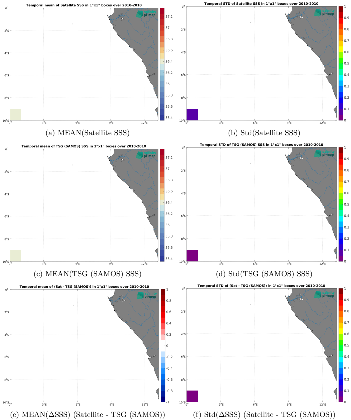
Figure 7: Temporal mean (left) and Std (right) of SSS from SMOS SSS L2Q v331 - No FLAG (CMEMS-CATDS-CPDC) (top), TSG (SAMOS) (middle), and of \Delta SSS (Satellite - TSG (SAMOS)). Only match-up pairs are used to generate these maps.
