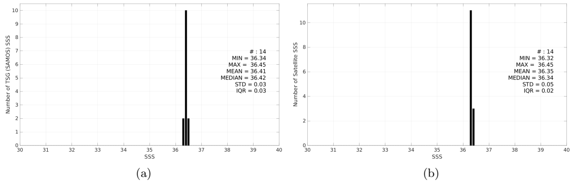
Figure 3: Histograms of SSS from TSG (SAMOS) (a) and SMOS SSS L2Q v331 - No FLAG (CMEMS-CATDS-CPDC) (b) considering all match-up pairs per bins of 0.1 over the Congo river plume Pi-MEP region and for the full satellite product period.
