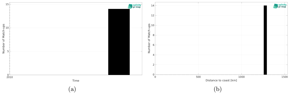
Figure 2: Number of match-ups between TSG (SAMOS) and SMOS SSS L2Q v331 - No FLAG (CMEMS-CATDS-CPDC) SSS as a function of time (a) and as function of the distance to coast (b) over the Congo river plume Pi-MEP region and for the full satellite product period.
