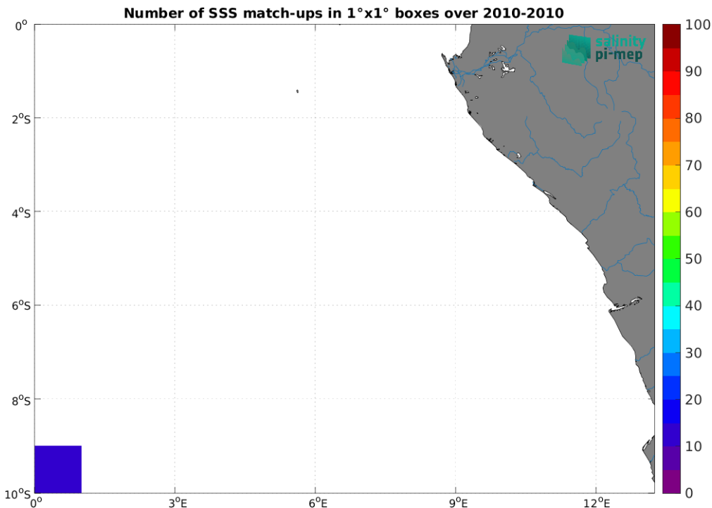
Figure 5: Number of SSS match-ups between TSG (SAMOS) SSS and the SMOS SSS L2Q v331 - No FLAG (CMEMS-CATDS-CPDC) SSS product for the Congo river plume Pi-MEP region over 1^\circ \times 1^\circ boxes and for the full satellite product period.
