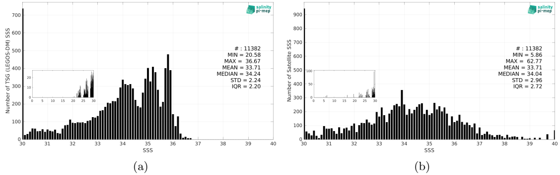
Figure 3: Histograms of SSS from TSG (LEGOS-DM) (a) and SMOS SSS L2Q v331 - No FLAG (CMEMS-CATDS-CPDC) (b) considering all match-up pairs per bins of 0.1 over the Congo river plume Pi-MEP region and for the full satellite product period.
