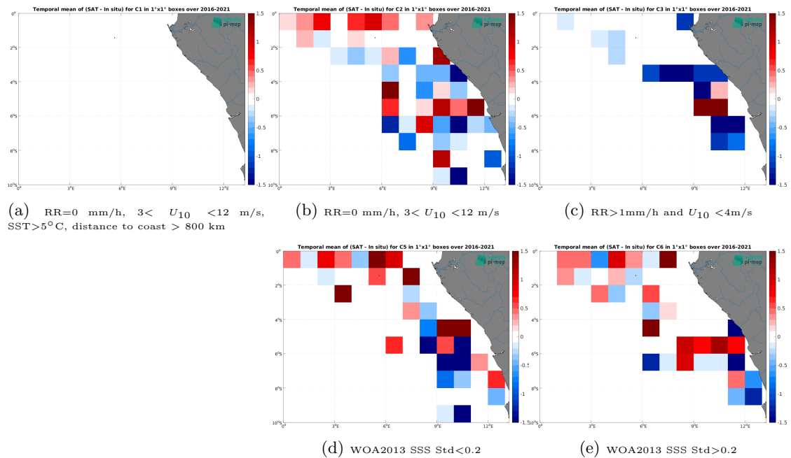
Figure 14: Temporal mean gridded over spatial boxes of size 1^\circ \times 1^\circ of \Delta SSS (SMOS SSS L2Q v331 - No FLAG (CMEMS-CATDS-CPDC) - TSG (LEGOS-DM)) for 5 different subdatasets corresponding to:RR=0 mm/h, 3 < U_{10} < 12 m/s, SST > 5^\circ\text{C} , distance to coast > 800 km (a), RR=0 mm/h, 3 < U_{10} < 12 m/s (b), RR > 1 mm/h and U_{10} < 4 m/s (c), WOA2013 SSS Std < 0.2 (d), WOA2013 SSS Std > 0.2 (e).
