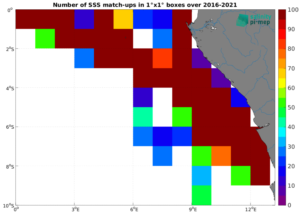
Figure 5: Number of SSS match-ups between TSG (LEGOS-DM) SSS and the SMOS SSS L2Q v331 - No FLAG (CMEMS-CATDS-CPDC) SSS product for the Congo river plume Pi-MEP region over 1^\circ \times 1^\circ boxes and for the full satellite product period.
