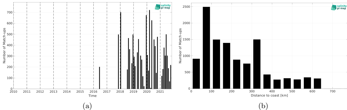
Figure 2: Number of match-ups between TSG (LEGOS-DM) and SMOS SSS L2Q v331 - No FLAG (CMEMS-CATDS-CPDC) SSS as a function of time (a) and as function of the distance to coast (b) over the Congo river plume Pi-MEP region and for the full satellite product period.
