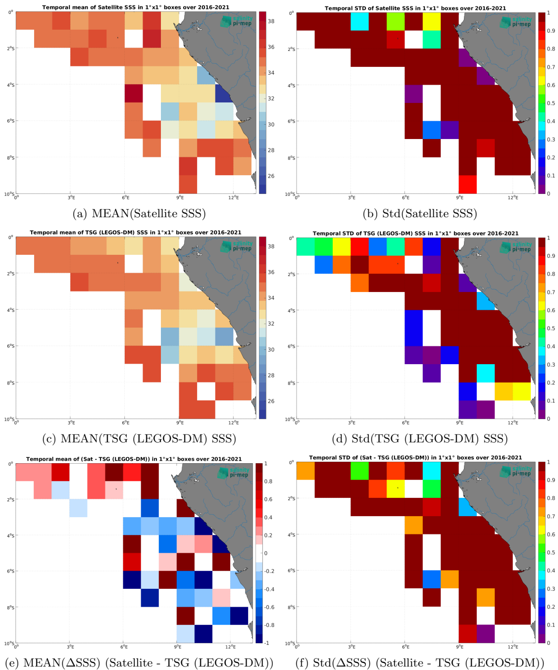
Figure 7: Temporal mean (left) and Std (right) of SSS from SMOS SSS L2Q v331 - No FLAG (CMEMS-CATDS-CPDC) (top), TSG (LEGOS-DM) (middle), and of \Delta SSS (Satellite - TSG (LEGOS-DM)). Only match-up pairs are used to generate these maps.
