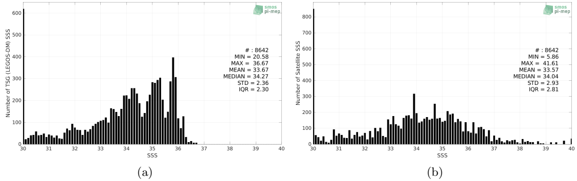
Figure 2: Histograms of SSS from TSG (LEGOS-DM) (a) and SMOS SSS L2Q v331 - No FLAG (CMEMS-CATDS-CPDC) (b) considering all match-up pairs per bins of 0.1 over the Congo river plume Pi-MEP region and for the full satellite product period.
