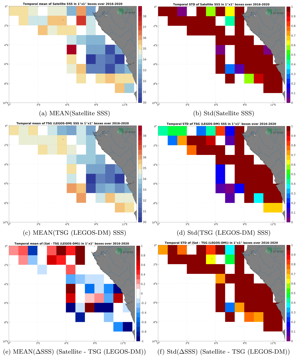
Figure 6: Temporal mean (left) and Std (right) of SSS from SMOS SSS L2Q v331 - No FLAG (CMEMS-CATDS-CPDC) (top), TSG (LEGOS-DM) (middle), and of \Delta SSS (Satellite - TSG (LEGOS-DM)). Only match-up pairs are used to generate these maps.
