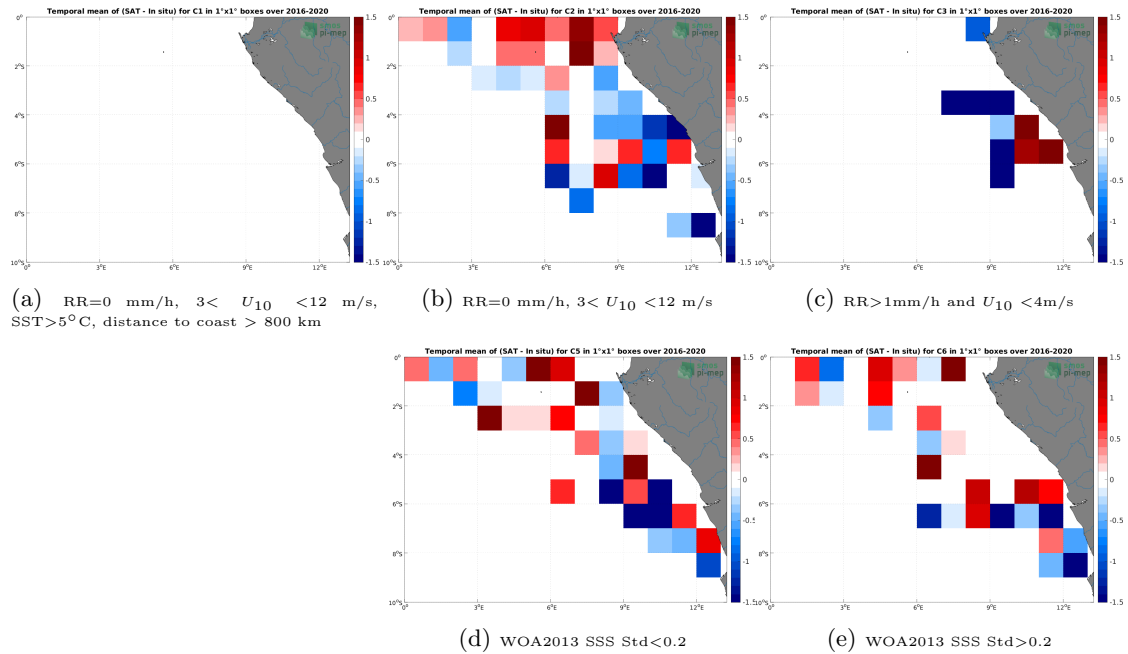
Figure 12: Temporal mean gridded over spatial boxes of size 1^{\circ}\times 1^{\circ} of \Delta\text{SSS} (SMOS SSS L2Q v331 - No FLAG (CMEMS-CATDS-CPDC) - TSG (LEGOS-DM)) for 5 different subdatasets corresponding to:RR=0 mm/h, 3 < U_{10} < 12 m/s, SST >5^{\circ}\text{C} , distance to coast > 800 km (a), RR=0 mm/h, 3 < U_{10} < 12 m/s (b), RR >1 mm/h and U_{10} < 4 m/s (c), WOA2013 SSS Std <0.2 (d), WOA2013 SSS Std >0.2 (e).
