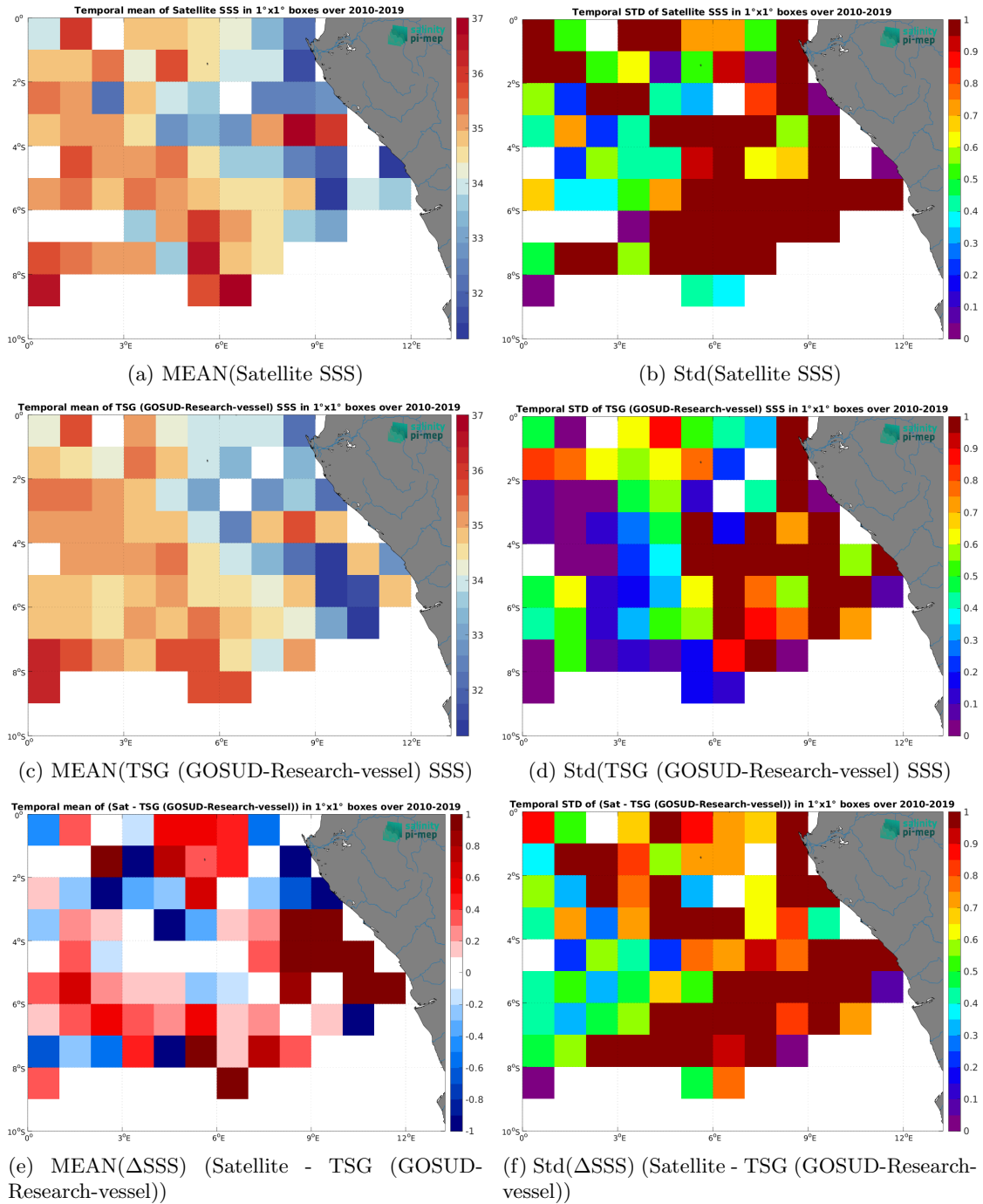
Figure 7: Temporal mean (left) and Std (right) of SSS from SMOS SSS L2Q v331 - No FLAG (CMEMS-CATDS-CPDC) (top), TSG (GOSUD-Research-vessel) (middle), and of \Delta SSS (Satellite - TSG (GOSUD-Research-vessel)). Only match-up pairs are used to generate these maps.
