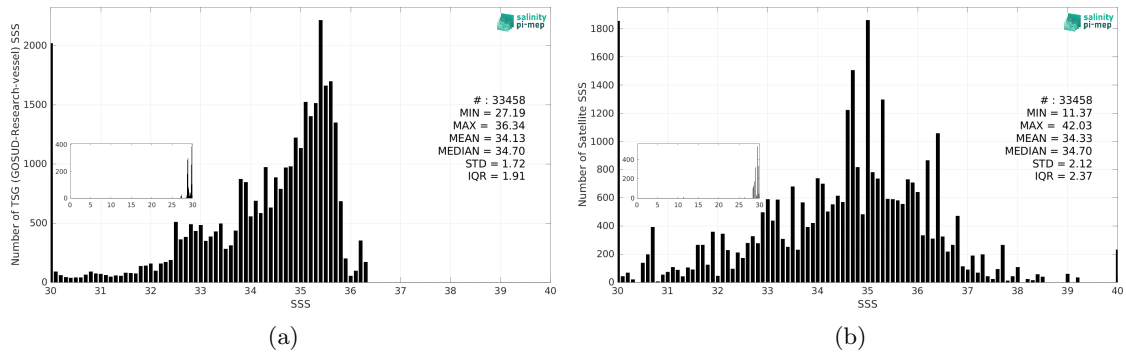
Figure 3: Histograms of SSS from TSG (GOSUD-Research-vessel) (a) and SMOS SSS L2Q v331 - No FLAG (CMEMS-CATDS-CPDC) (b) considering all match-up pairs per bins of 0.1 over the Congo river plume Pi-MEP region and for the full satellite product period.
