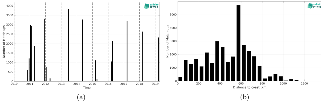
Figure 2: Number of match-ups between TSG (GOSUD-Research-vessel) and SMOS SSS L2Q v331 - No FLAG (CMEMS-CATDS-CPDC) SSS as a function of time (a) and as function of the distance to coast (b) over the Congo river plume Pi-MEP region and for the full satellite product period.
