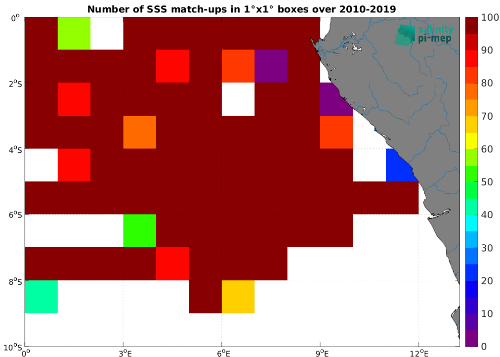
Figure 5: Number of SSS match-ups between TSG (GOSUD-Research-vessel) SSS and the SMOS SSS L2Q v331 - No FLAG (CMEMS-CATDS-CPDC) SSS product for the Congo river plume Pi-MEP region over 1^\circ \times 1^\circ boxes and for the full satellite product period.
