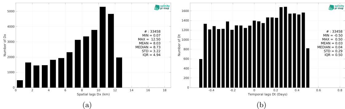
Figure 6: Histograms of the spatial (a) and temporal (b) lags between the location/time of the TSG (GOSUD-Research-vessel) measurement and the date of the corresponding SMOS SSS L2Q v331 - No FLAG (CMEMS-CATDS-CPDC) SSS pixel.
