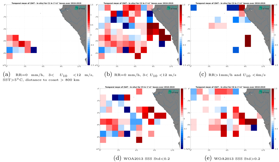
Figure 14: Temporal mean gridded over spatial boxes of size 1^\circ \times 1^\circ of \Delta SSS (SMOS SSS L2Q v331 - No FLAG (CMEMS-CATDS-CPDC) - TSG (GOSUD-Research-vessel)) for 5 different subdatasets corresponding to:RR=0 mm/h, 3 < U_{10} < 12 m/s, SST > 5^\circ\text{C} , distance to coast > 800 km (a), RR=0 mm/h, 3 < U_{10} < 12 m/s (b), RR > 1 mm/h and U_{10} < 4 m/s (c), WOA2013 SSS Std < 0.2 (d), WOA2013 SSS Std > 0.2 (e).
