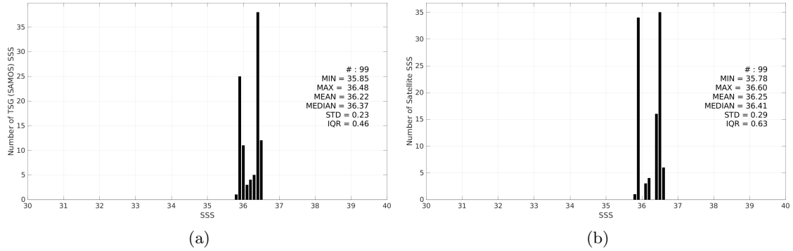
Figure 2: Histograms of SSS from TSG (SAMOS) (a) and SMOS SSS L3 v9 - 9 Days (CATDS-CEC-LOCEAN) (b) considering all match-up pairs per bins of 0.1 over the Congo river plume Pi-MEP region and for the full satellite product period.
