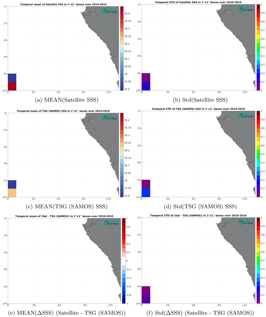
Figure 6: Temporal mean (left) and Std (right) of SSS from SMOS SSS L3 v9 - 9 Days (CATDS-CEC-LOCEAN) (top), TSG (SAMOS) (middle), and of \Delta SSS (Satellite - TSG (SAMOS)). Only match-up pairs are used to generate these maps.
