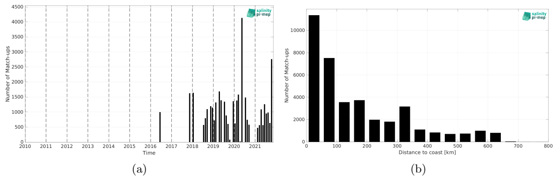
Figure 1: Number of match-ups between TSG (LEGOS-DM) and SMOS SSS L3 v9 - 9 Days (CATDS-CEC-LOCEAN) SSS as a function of time (a) and as function of the distance to coast (b) over the Congo river plume Pi-MEP region and for the full satellite product period.
