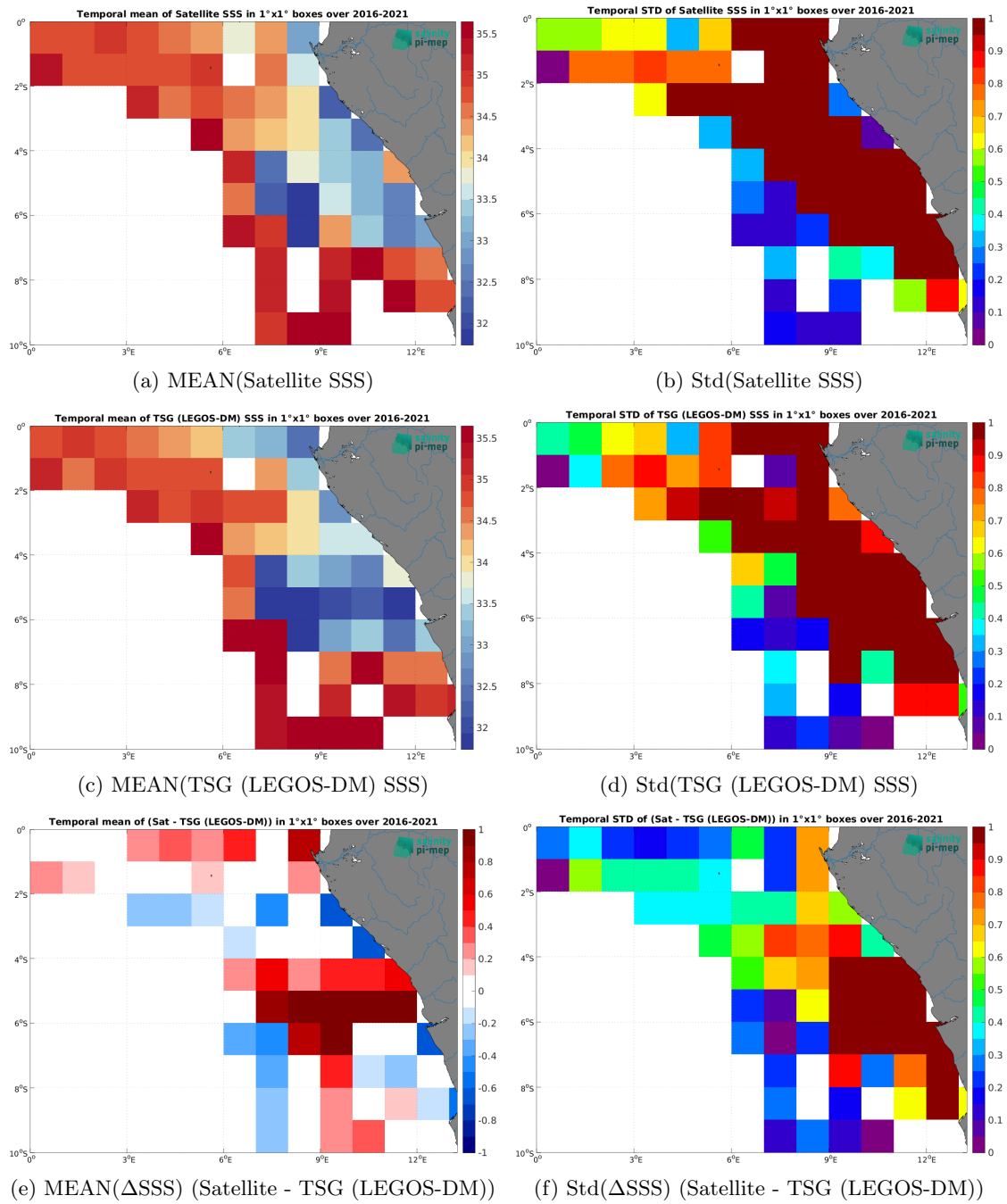
Figure 6: Temporal mean (left) and Std (right) of SSS from SMOS SSS L3 v9 - 9 Days (CATDS-CEC-LOCEAN) (top), TSG (LEGOS-DM) (middle), and of \Delta SSS (Satellite - TSG (LEGOS-DM)). Only match-up pairs are used to generate these maps.
