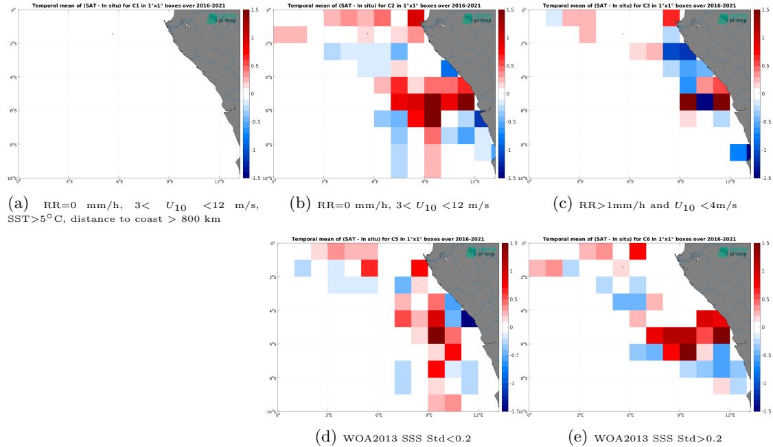
Figure 12: Temporal mean gridded over spatial boxes of size 1^{\circ}\times 1^{\circ} of \Delta\text{SSS} (SMOS SSS L3 v9 - 9 Days (CATDS-CEC-LOCEAN) - TSG (LEGOS-DM)) for 5 different subdatasets corresponding to:RR=0 mm/h, 3 < U_{10} < 12 m/s, SST >5^{\circ}\text{C} , distance to coast > 800 km (a), RR=0 mm/h, 3 < U_{10} < 12 m/s (b), RR >1 mm/h and U_{10} < 4 m/s (c), WOA2013 SSS Std <0.2 (d), WOA2013 SSS Std >0.2 (e).
