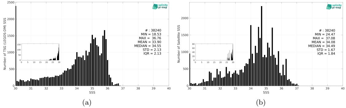
Figure 2: Histograms of SSS from TSG (LEGOS-DM) (a) and SMOS SSS L3 v9 - 9 Days (CATDS-CEC-LOCEAN) (b) considering all match-up pairs per bins of 0.1 over the Congo river plume Pi-MEP region and for the full satellite product period.
