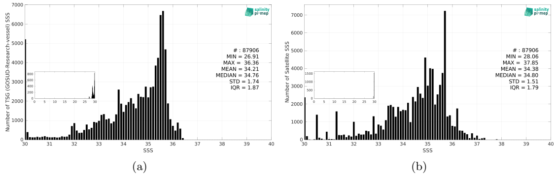
Figure 3: Histograms of SSS from TSG (GOSUD-Research-vessel) (a) and SMOS SSS L3 v9 - 9 Days (CATDS-CEC-LOCEAN) (b) considering all match-up pairs per bins of 0.1 over the Congo river plume Pi-MEP region and for the full satellite product period.
