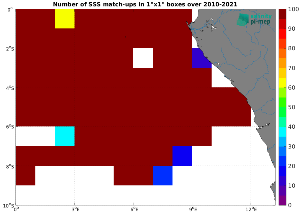
Figure 5: Number of SSS match-ups between TSG (GOSUD-Research-vessel) SSS and the SMOS SSS L3 v9 - 9 Days (CATDS-CEC-LOCEAN) SSS product for the Congo river plume Pi-MEP region over 1^\circ \times 1^\circ boxes and for the full satellite product period.
