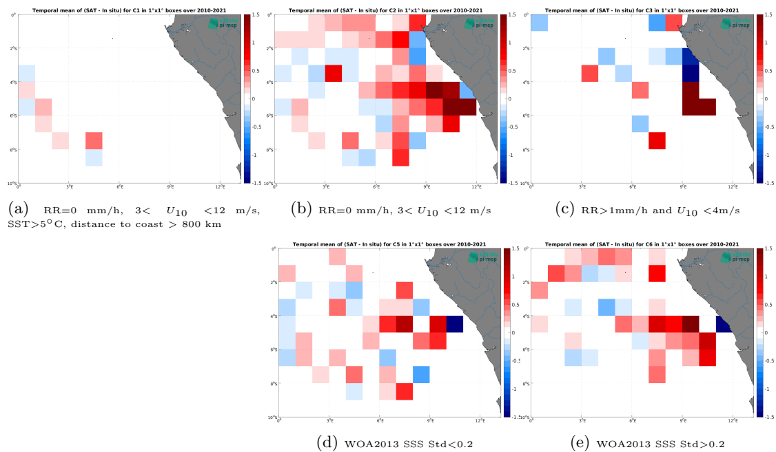
Figure 14: Temporal mean gridded over spatial boxes of size 1^\circ \times 1^\circ of \Delta SSS (SMOS SSS L3 v9 - 9 Days (CATDS-CEC-LOCEAN) - TSG (GOSUD-Research-vessel)) for 5 different subdatasets corresponding to:RR=0 mm/h, 3 < U_{10} < 12 m/s, SST > 5^\circ\text{C} , distance to coast > 800 km (a), RR=0 mm/h, 3 < U_{10} < 12 m/s (b), RR > 1 mm/h and U_{10} < 4 m/s (c), WOA2013 SSS Std < 0.2 (d), WOA2013 SSS Std > 0.2 (e).
