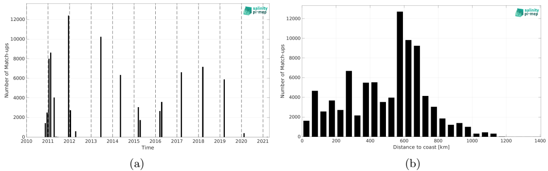
Figure 1: Number of match-ups between TSG (GOSUD-Research-vessel) and SMOS SSS L3 v9 - 9 Days (CATDS-CEC-LOCEAN) SSS as a function of time (a) and as function of the distance to coast (b) over the Congo river plume Pi-MEP region and for the full satellite product period.
