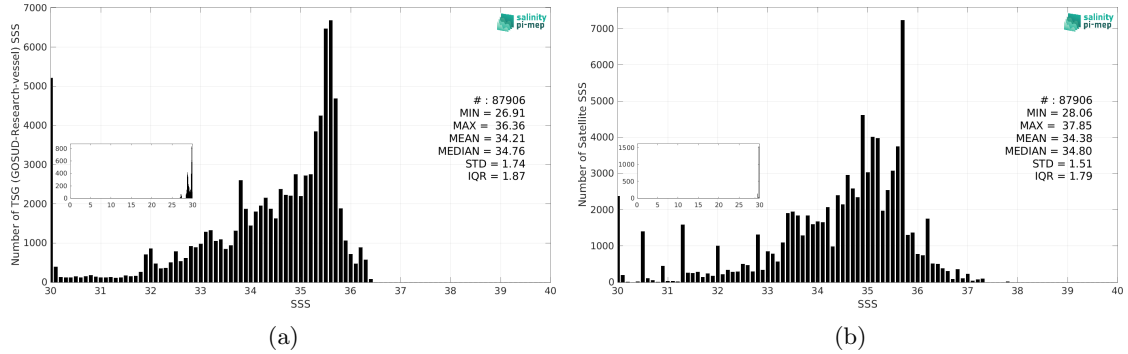
Figure 2: Histograms of SSS from TSG (GOSUD-Research-vessel) (a) and SMOS SSS L3 v9 - 9 Days (CATDS-CEC-LOCEAN) (b) considering all match-up pairs per bins of 0.1 over the Congo river plume Pi-MEP region and for the full satellite product period.
