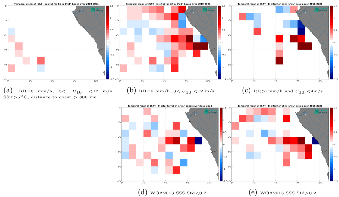
Figure 12: Temporal mean gridded over spatial boxes of size 1^\circ \times 1^\circ of \Delta SSS (SMOS SSS L3 v9 - 9 Days (CATDS-CEC-LOCEAN) - TSG (GOSUD-Research-vessel)) for 5 different subdatasets corresponding to:RR=0 mm/h, 3 < U_{10} < 12 m/s, SST > 5°C, distance to coast > 800 km (a), RR=0 mm/h, 3 < U_{10} < 12 m/s (b), RR > 1mm/h and U_{10} < 4 m/s (c), WOA2013 SSS Std < 0.2 (d), WOA2013 SSS Std > 0.2 (e).
