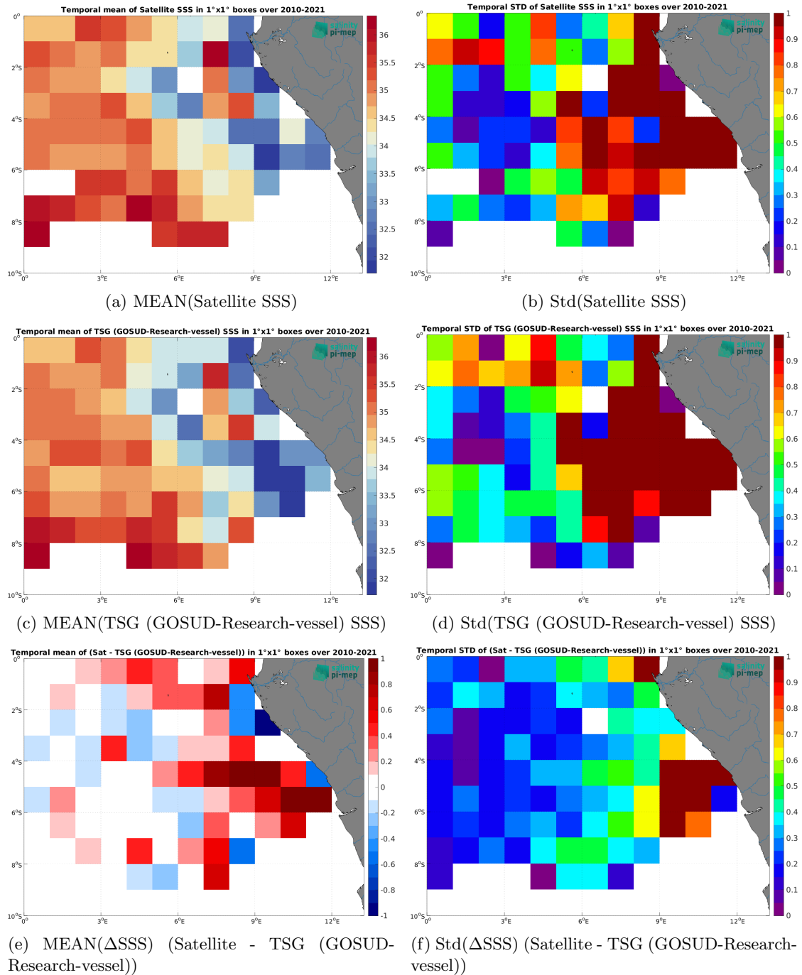
Figure 6: Temporal mean (left) and Std (right) of SSS from SMOS SSS L3 v9 - 9 Days (CATDS-CEC-LOCEAN) (top), TSG (GOSUD-Research-vessel) (middle), and of \Delta SSS (Satellite - TSG (GOSUD-Research-vessel)). Only match-up pairs are used to generate these maps.
